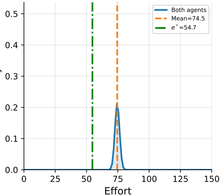
Step 131072 (10%) \kappa=3746.8
