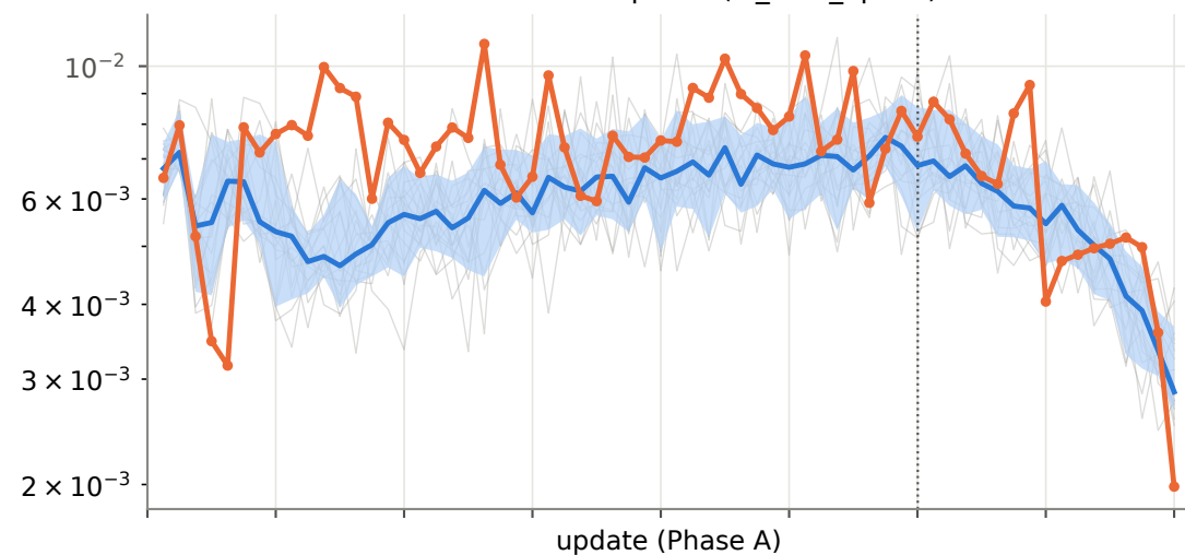
actor grad norm, pre-clip mean (clip level 0.5)
