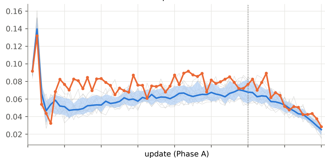
advantage SD (raw, before normalisation)
