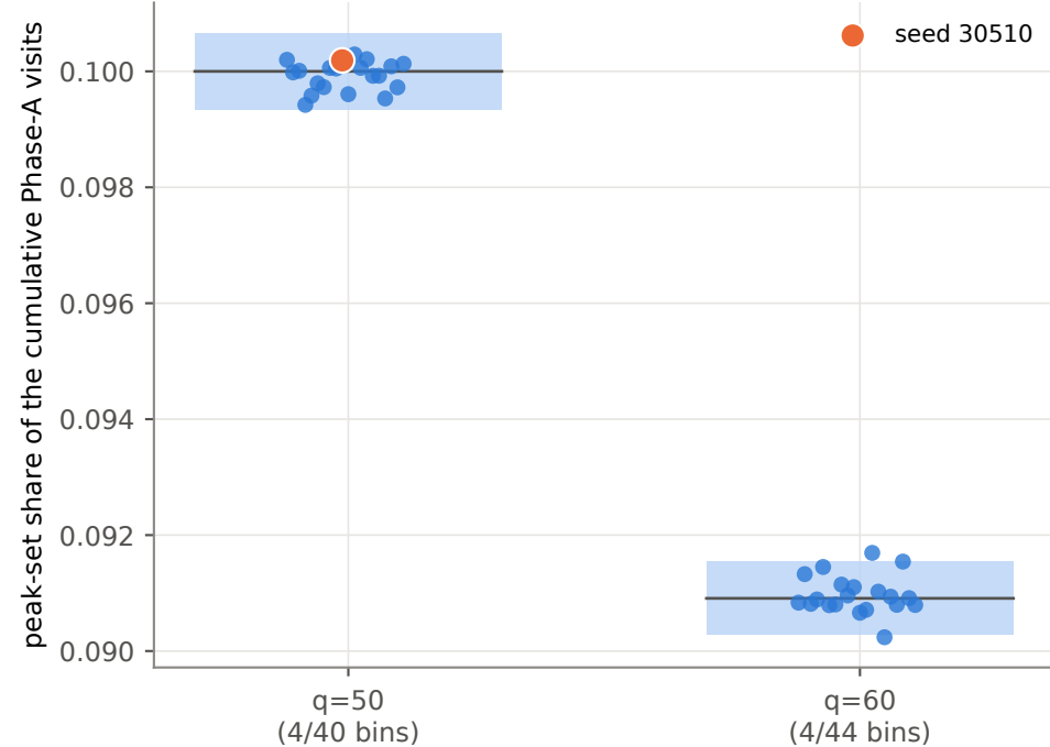
(a) share of visits in bins meeting (-20, 20) , u=1600 (band: \pm 2 binomial SD around the design value)
