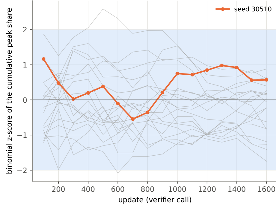
(b) cumulative peak-set share over Phase A (grey: other q=50 )
