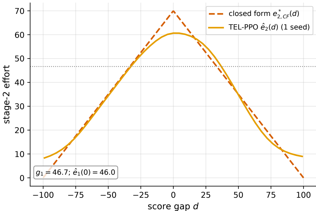
Two-stage equilibrium recovery ( T = 2 , q = 50 )
