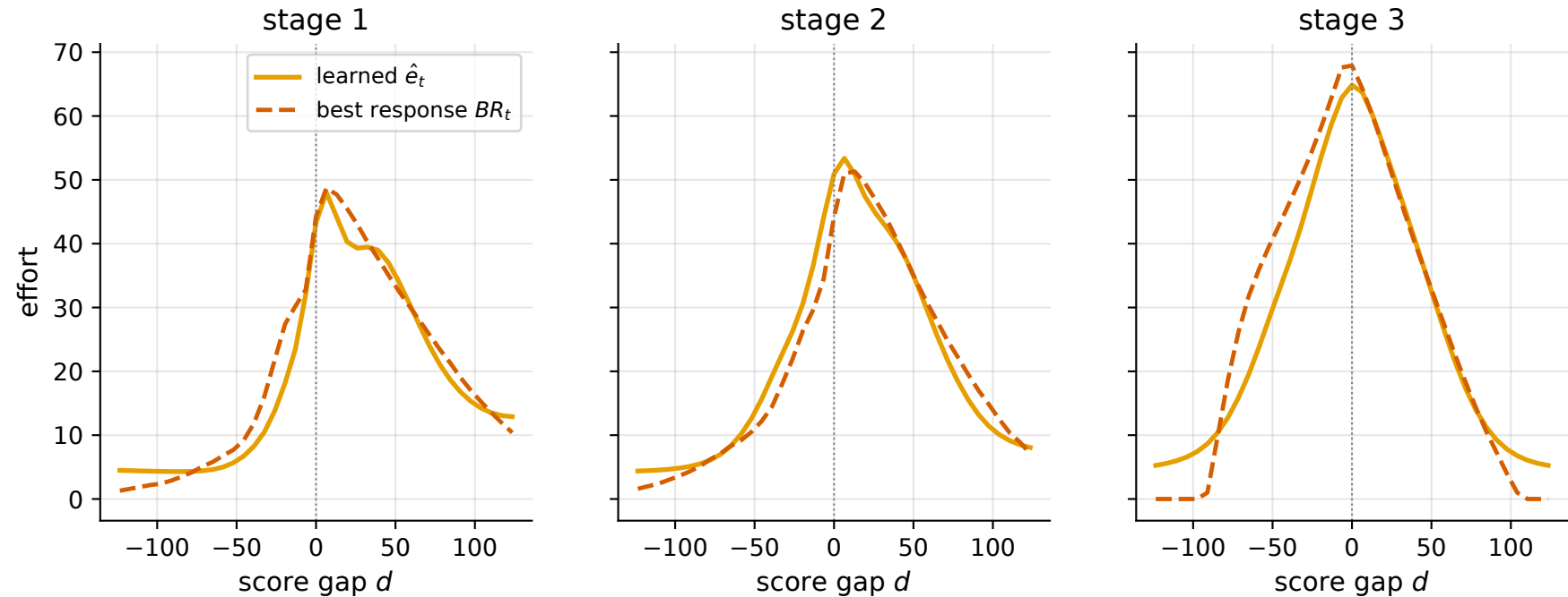
Three-stage best response vs learned effort ( T = 3 )
