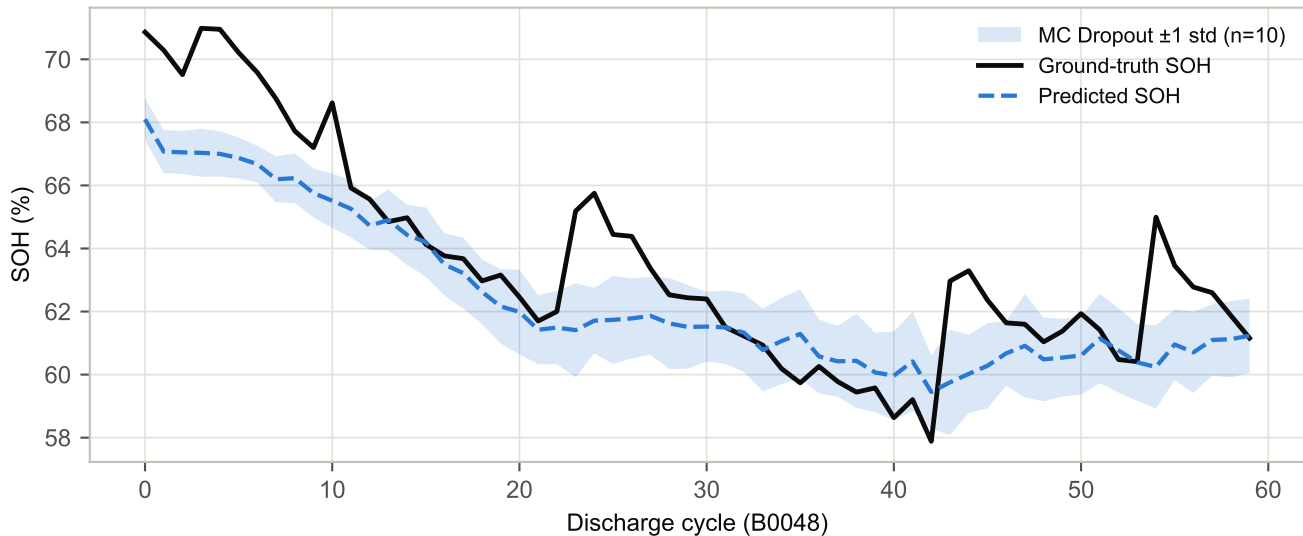
Predicted vs. true SOH on held-out B0048 — long model (MAE 1.52%, RMSE 1.97%)
