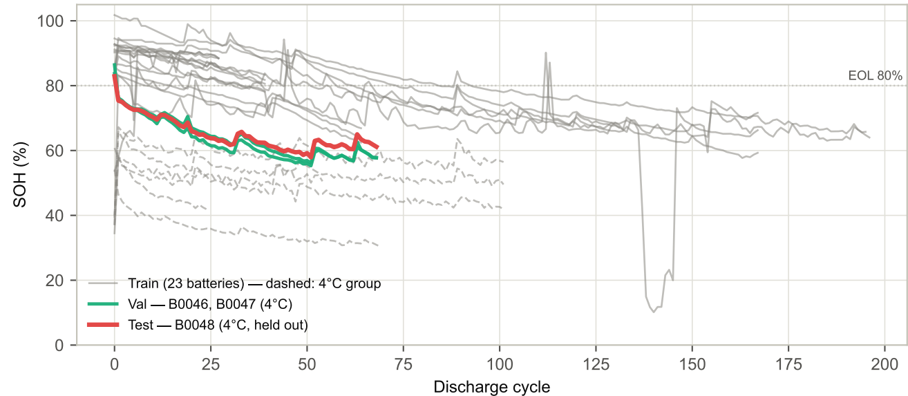
SOH degradation of the 26 NASA batteries, colored by split
