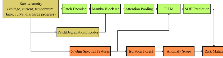
Fig. 1. Overall architecture of the proposed framework. Raw telemetry is encoded into patches and processed by two MambaBlocks; the pooled cycle representation is modulated by the 57-dimensional spectral feature vector via FiLM to produce the SOH estimate, while the same feature vector feeds an Isolation Forest whose anomaly score is combined with the SOH output in a rule-based risk matrix.
