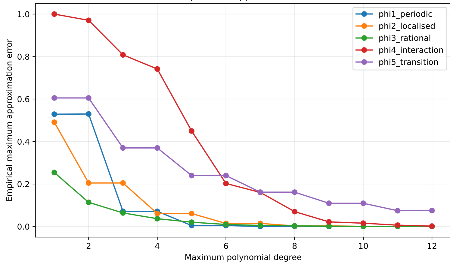
RQ1 expressive approximation (Linf)
