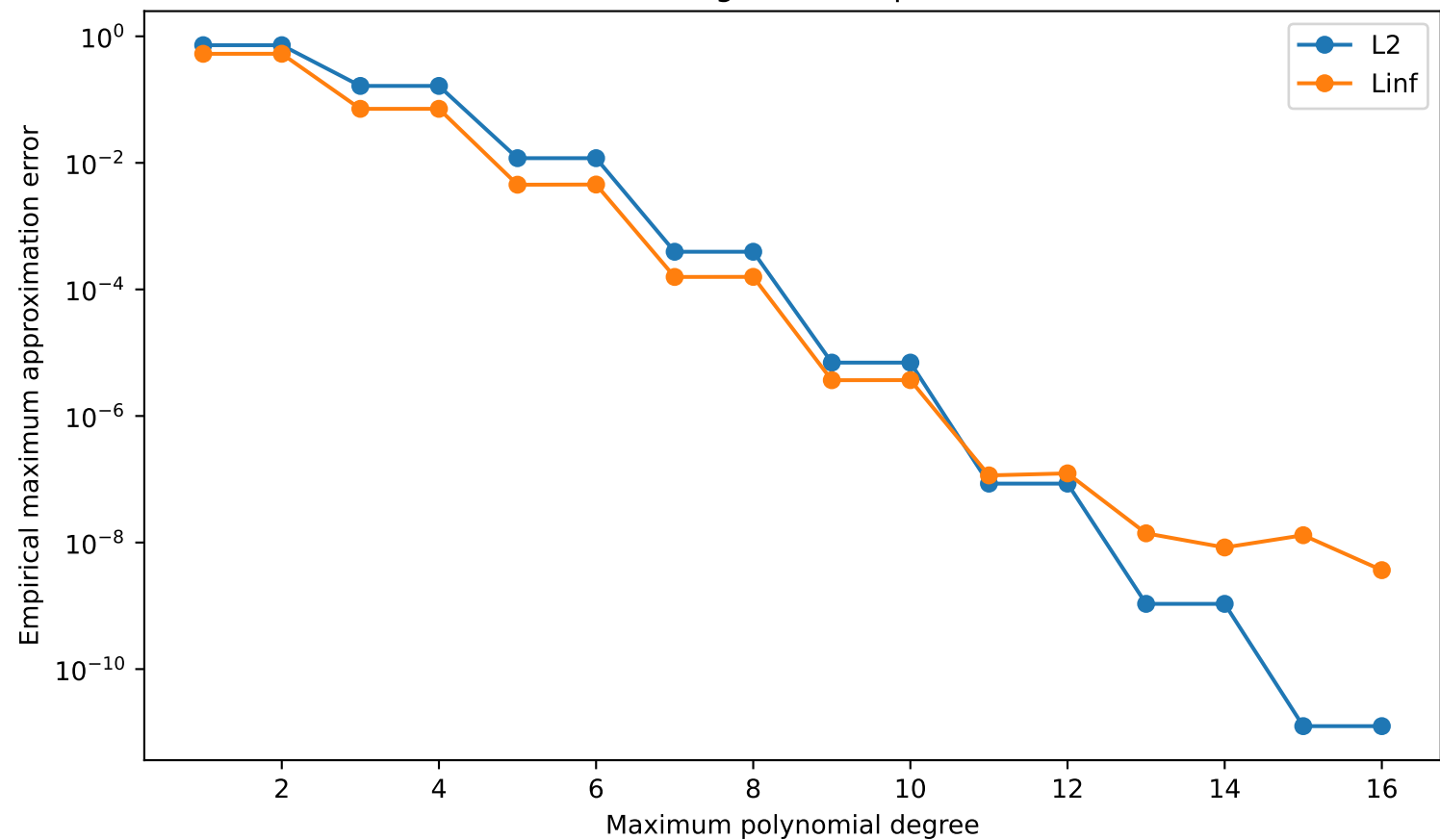
RQ1 fitting criterion: periodic
