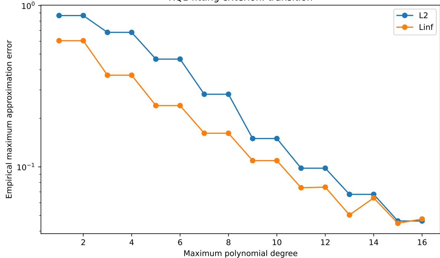
RQ1 fitting criterion: transition
