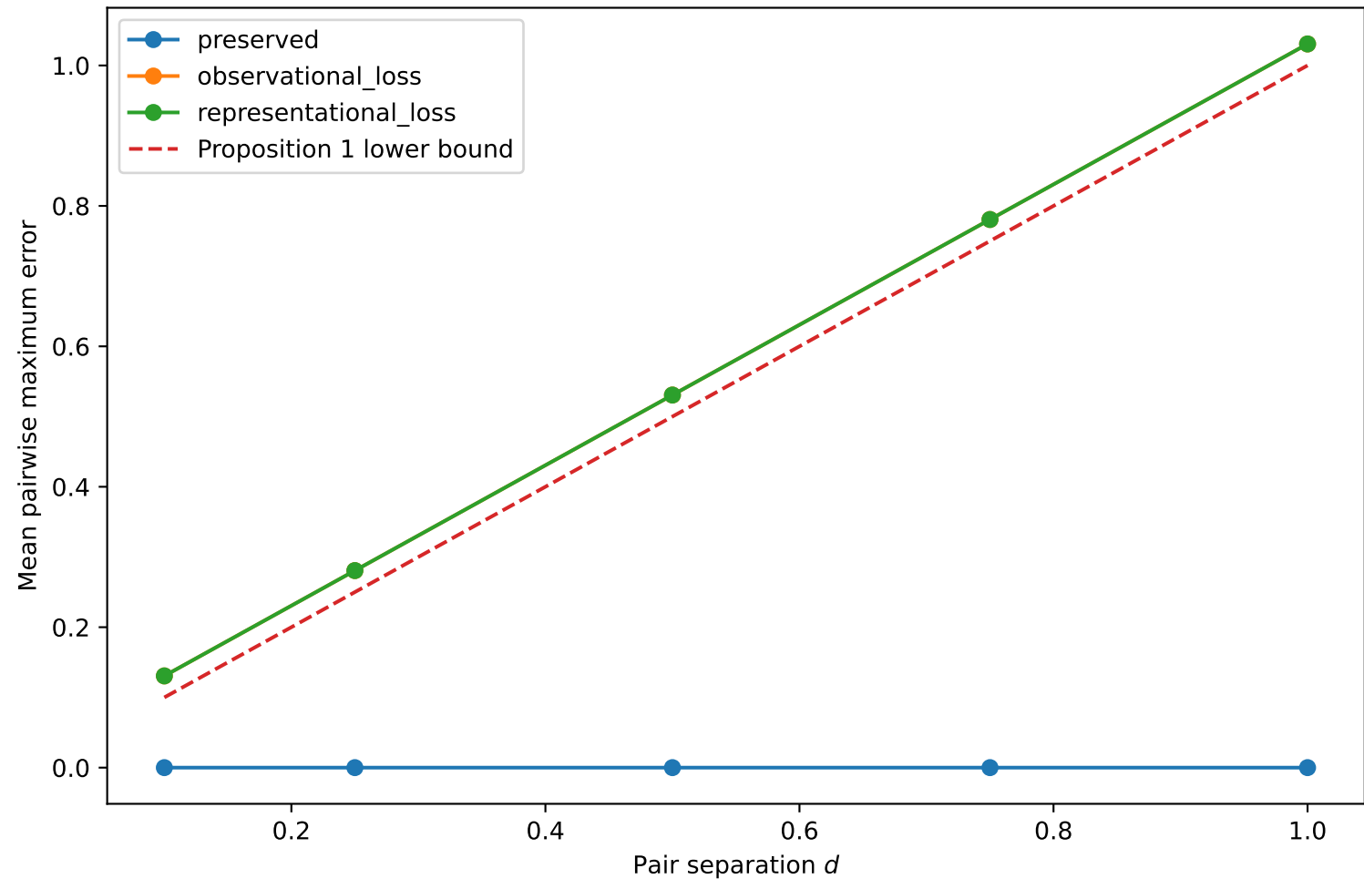
RQ2 pairwise approximation bound
