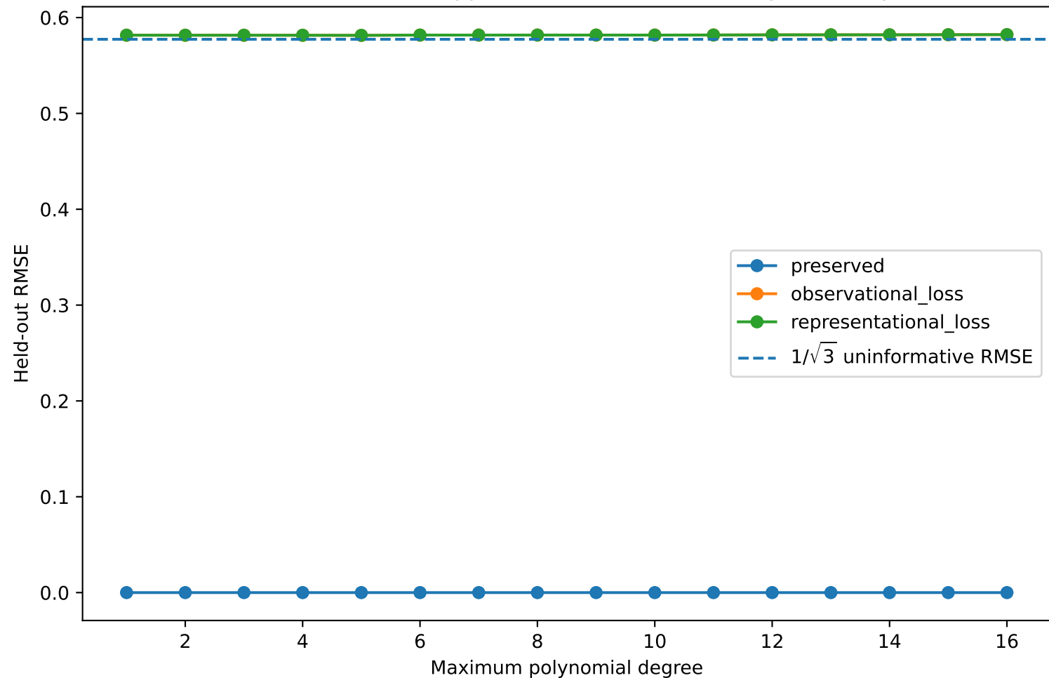
RQ2 downstream approximation under indistinguishability
