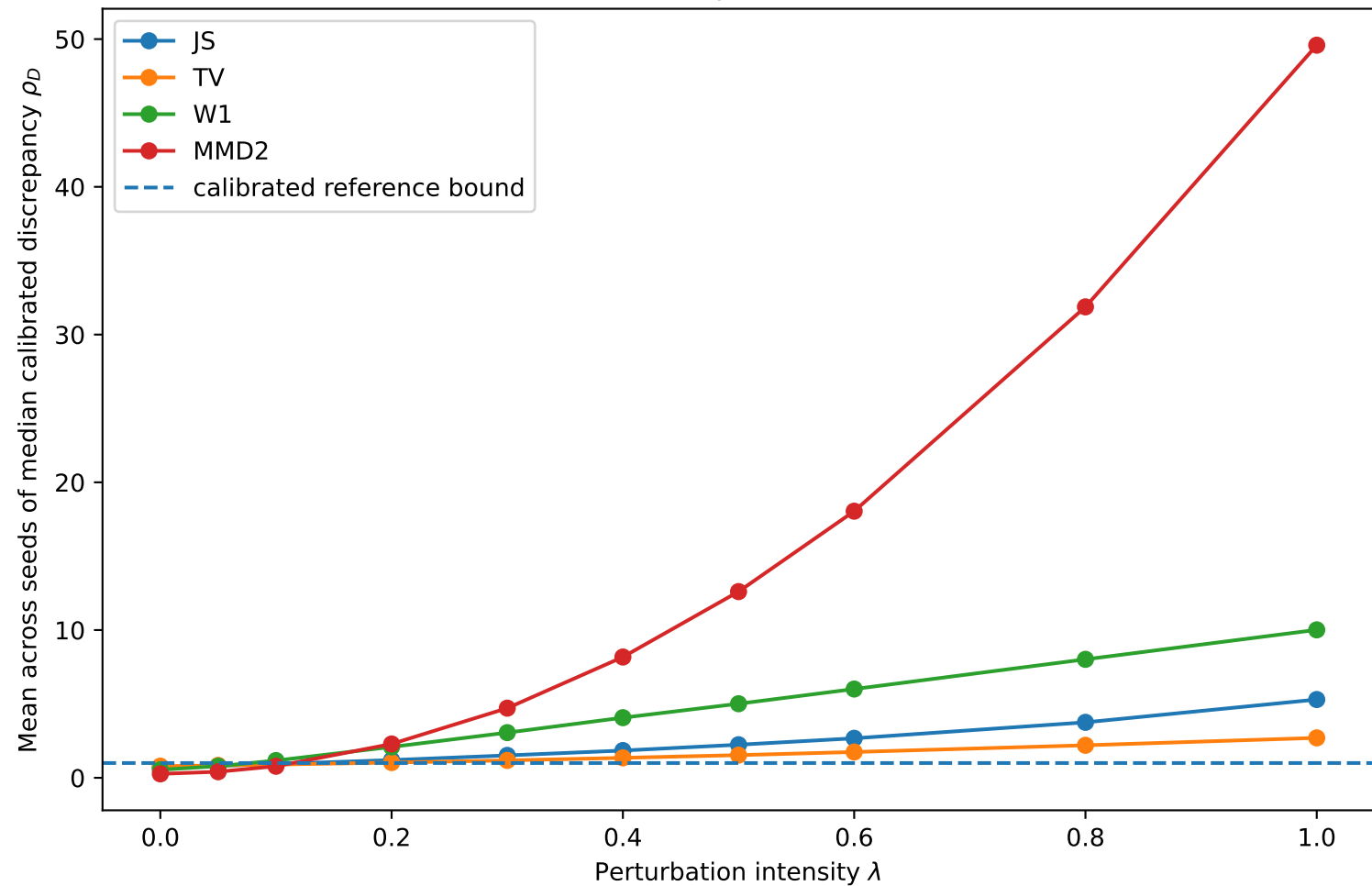
RQ3 calibrated response: contamination
