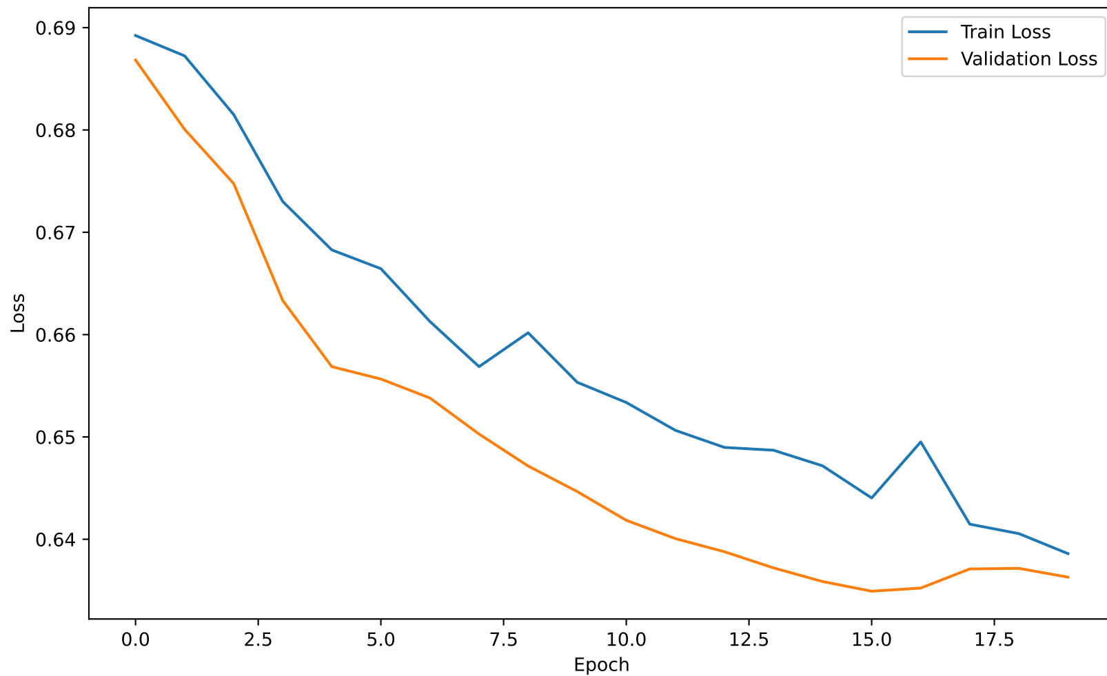
Loss - h=32, h2=16, lr=0.0001, bs=32
