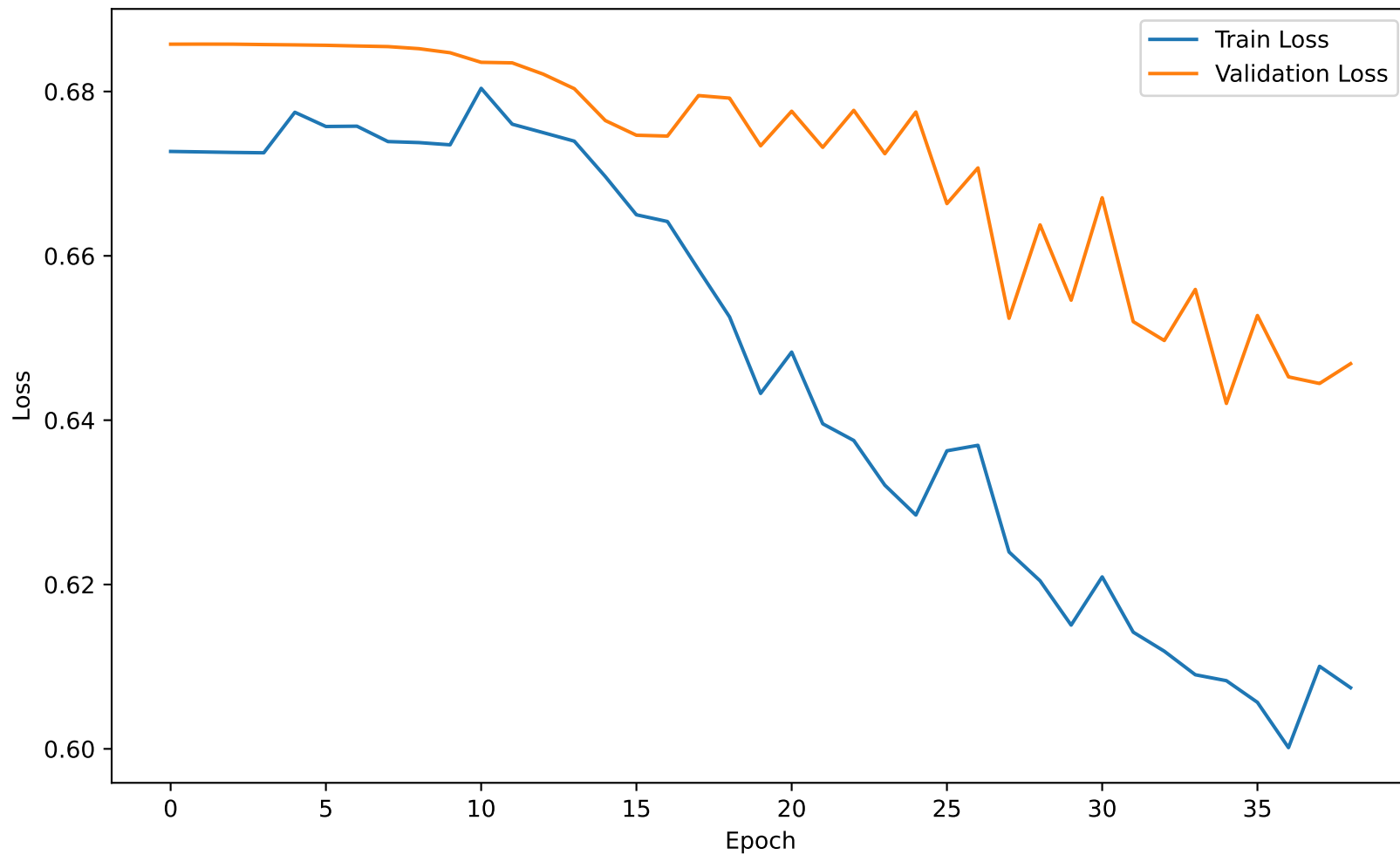
Loss - h=32, h2=16, lr=0.0001, bs=64
