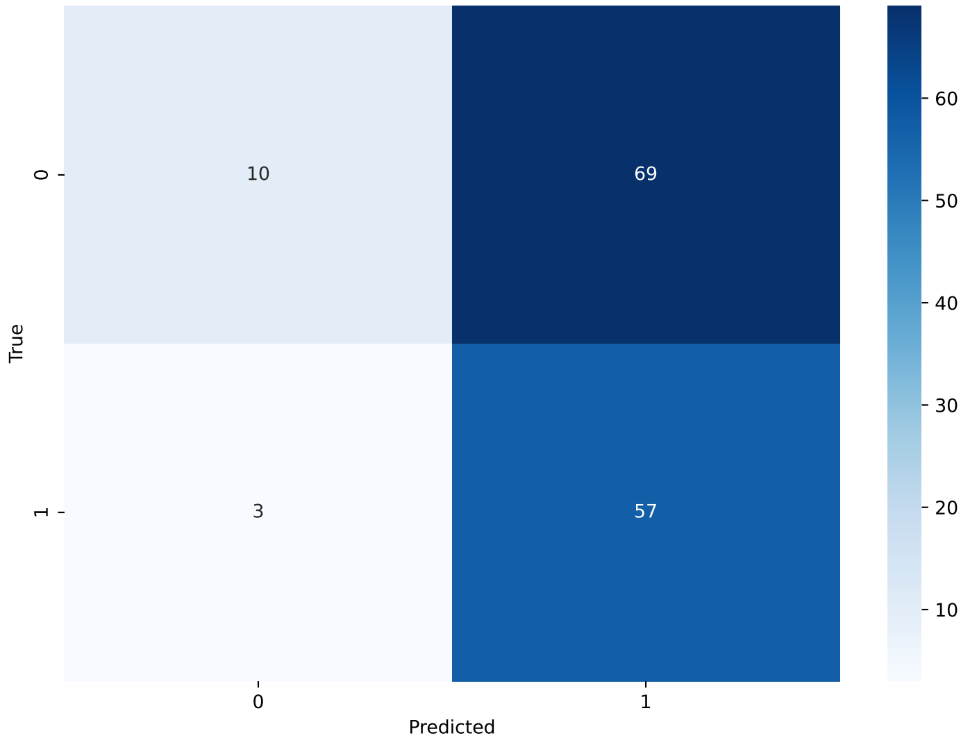
Confusion Matrix - h=32, h2=16, lr=0.0001, bs=64
