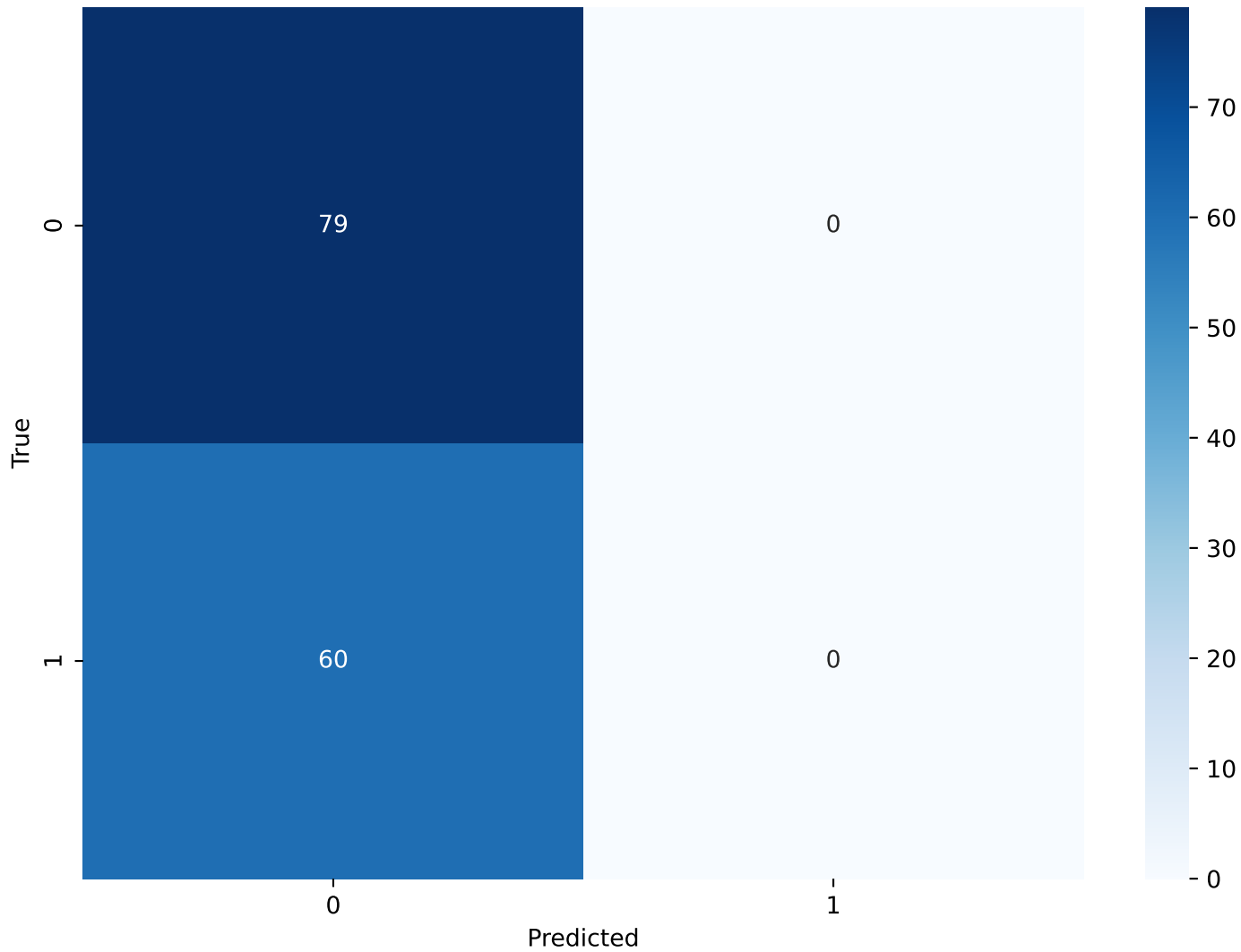
Confusion Matrix - h=32, h2=16, lr=0.01, bs=32
