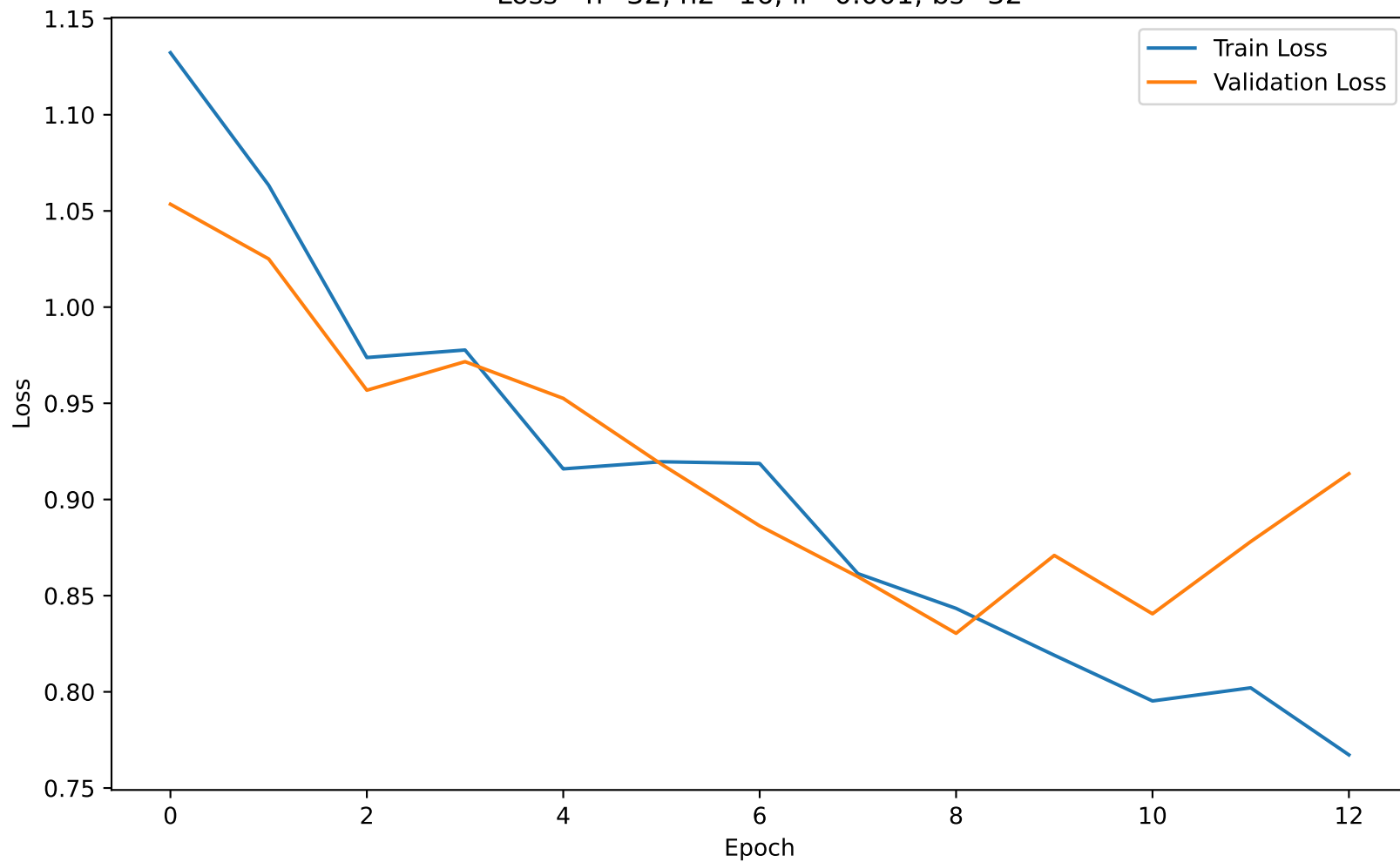
Loss - h=32, h2=16, lr=0.001, bs=32
