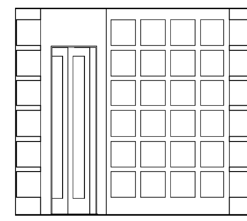
3 OFFICE - SOUTH 1/4" = 1'-0"
