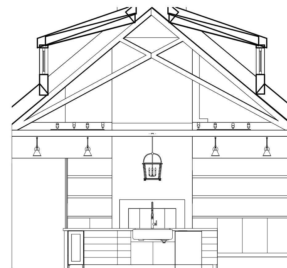
22 KITCHEN - EAST 1/4" = 1'-0"
