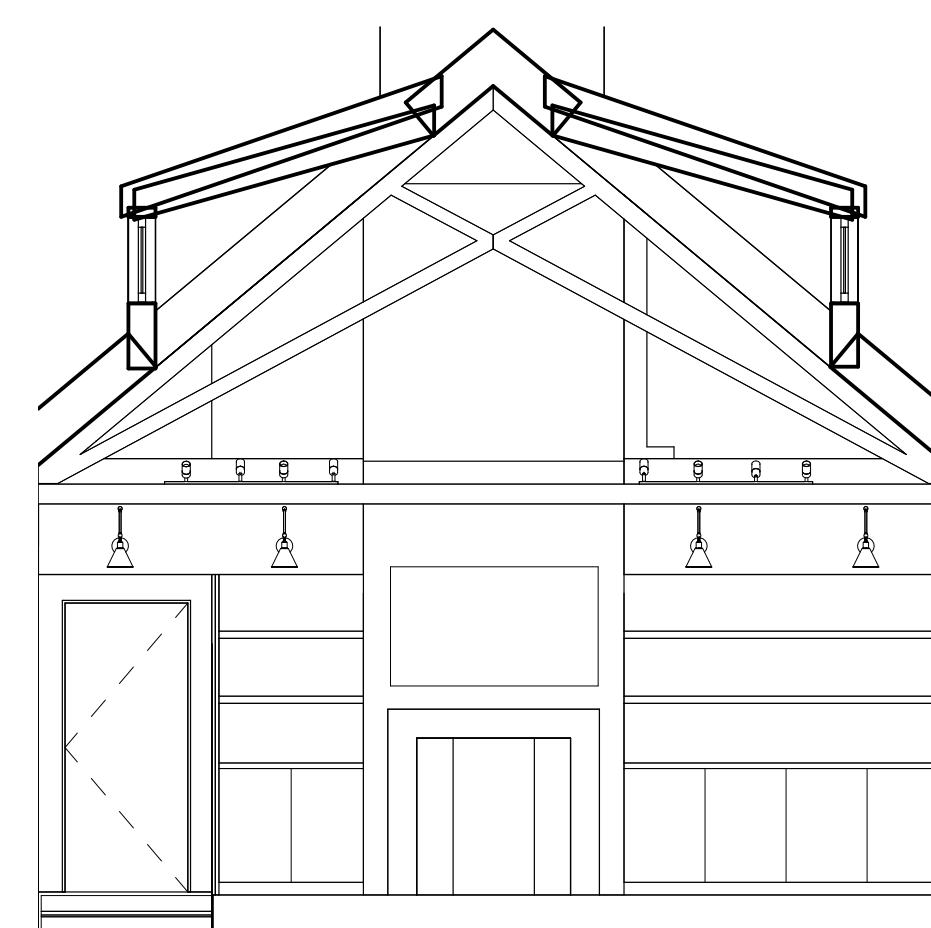
26 GREAT ROOM - EAST 1/4" = 1'-0"
