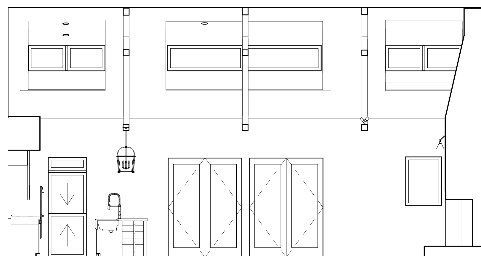
25 GREAT ROOM - NORTH 1/4" = 1'-0"
