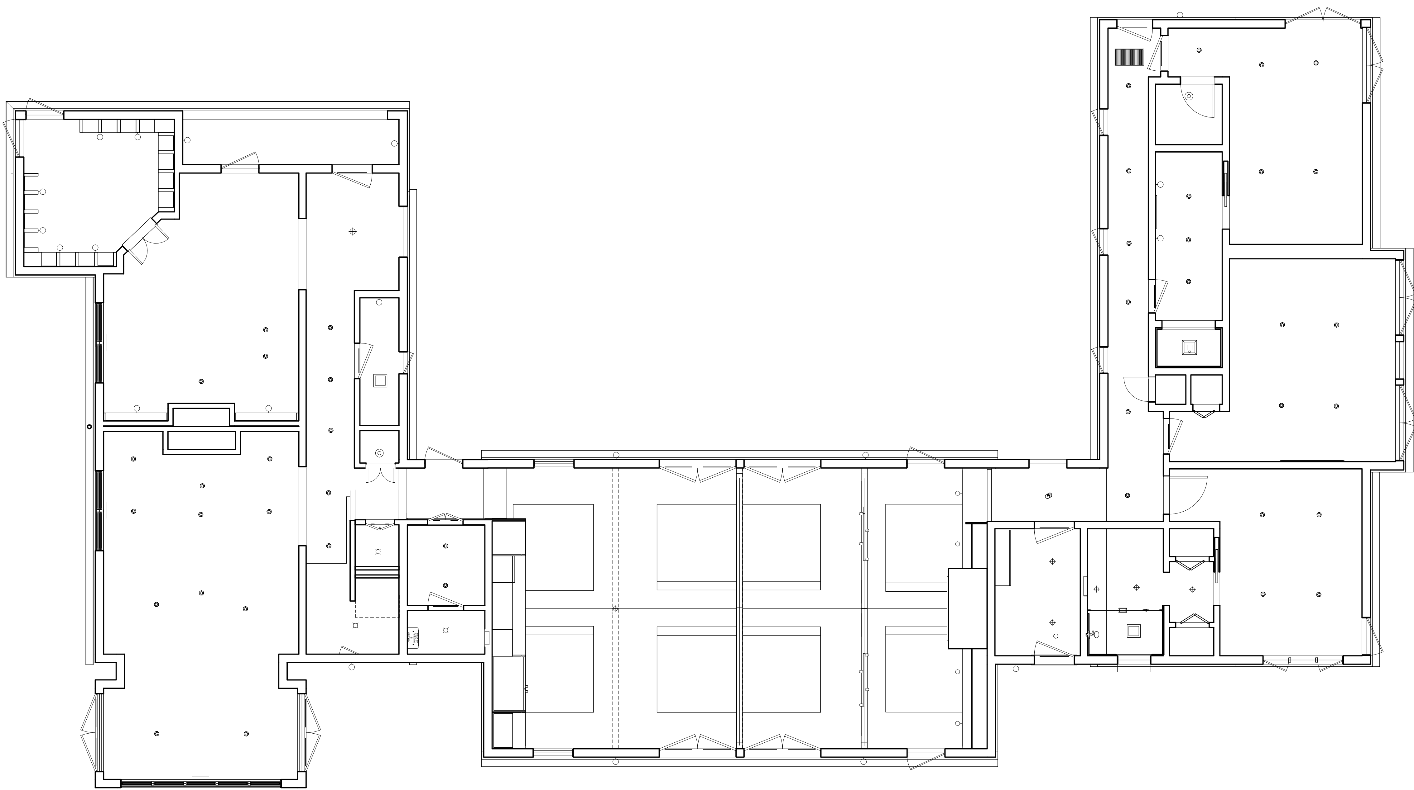
① LEVEL 1 1/4" = 1'-0"
