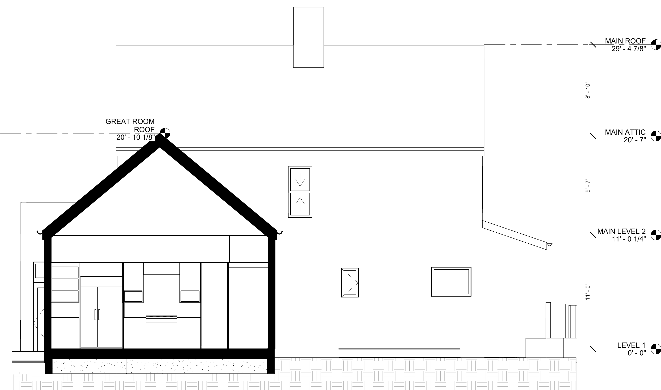
③ COURTYARD EAST 1/4" = 1'-0"
