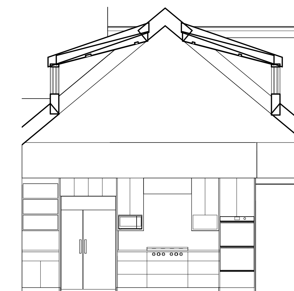
24 KITCHEN - WEST 1/4" = 1'-0"
