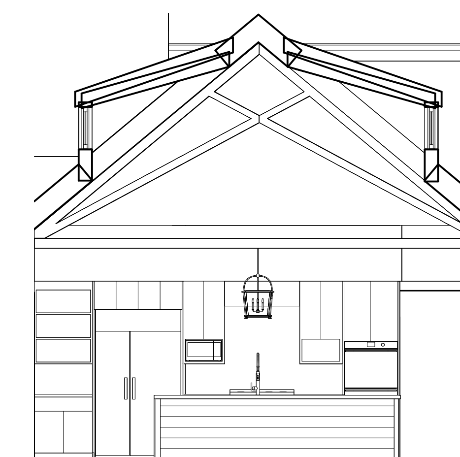
28 GREAT ROOM - WEST 1/4" = 1'-0"
