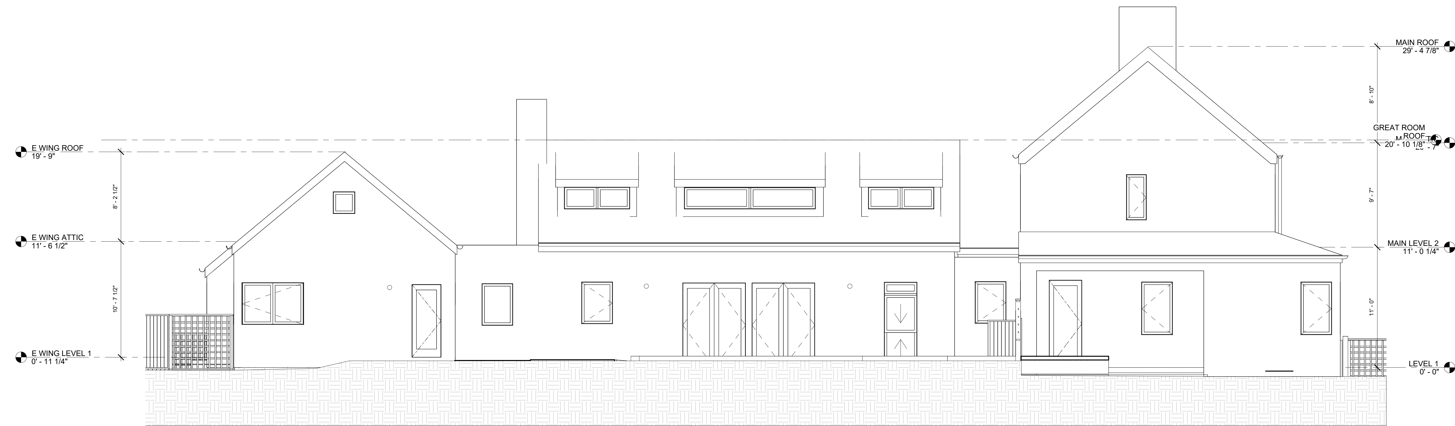
① NORTH ELEVATION 1/4" = 1'-0"
