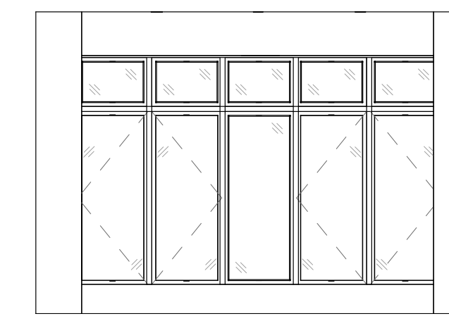
7 DINING ROOM - SOUTH 1/4" = 1'-0"
