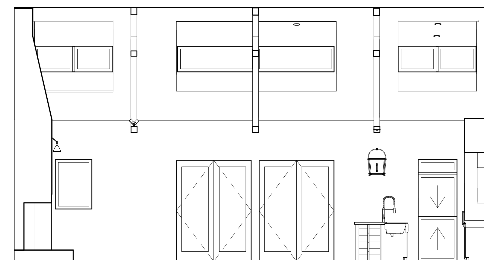
27 GREAT ROOM - SOUTH 1/4" = 1'-0"
