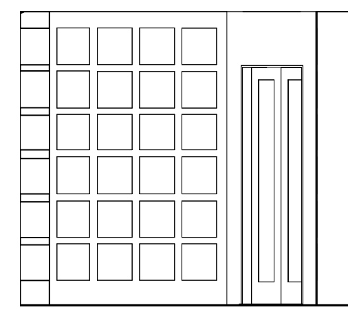
2 OFFICE - EAST 1/4" = 1'-0"
