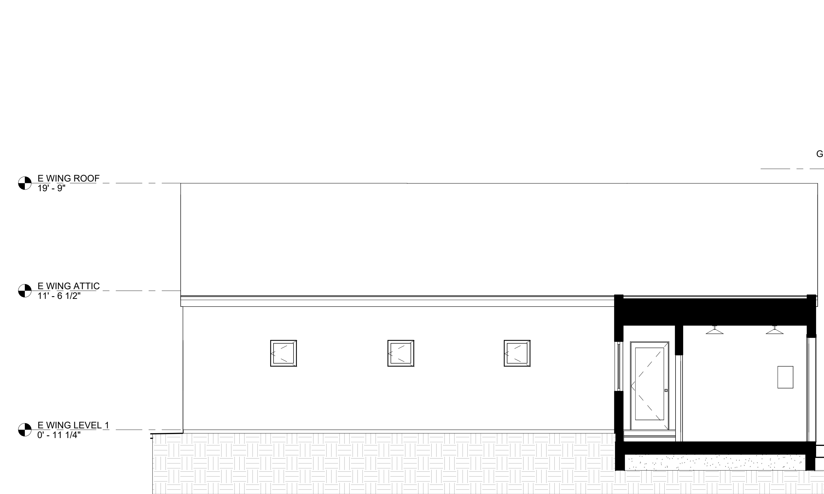
② COURTYARD WEST 1/4" = 1'-0"
