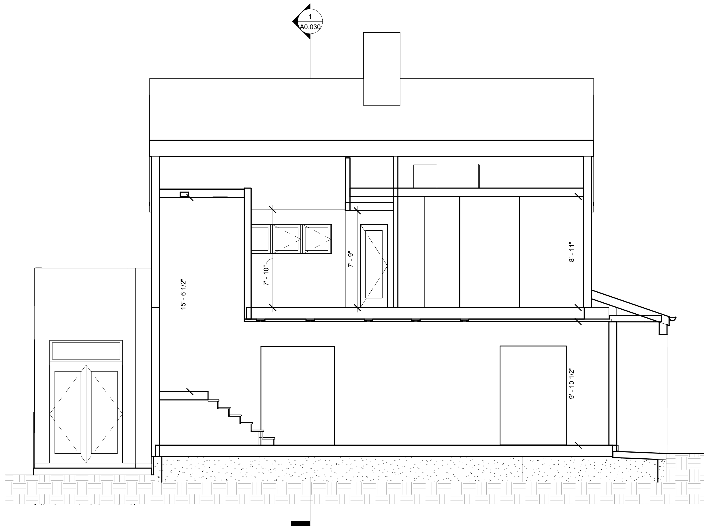
② MAIN - CROSS AT EAST WING 1/4" = 1'-0"
