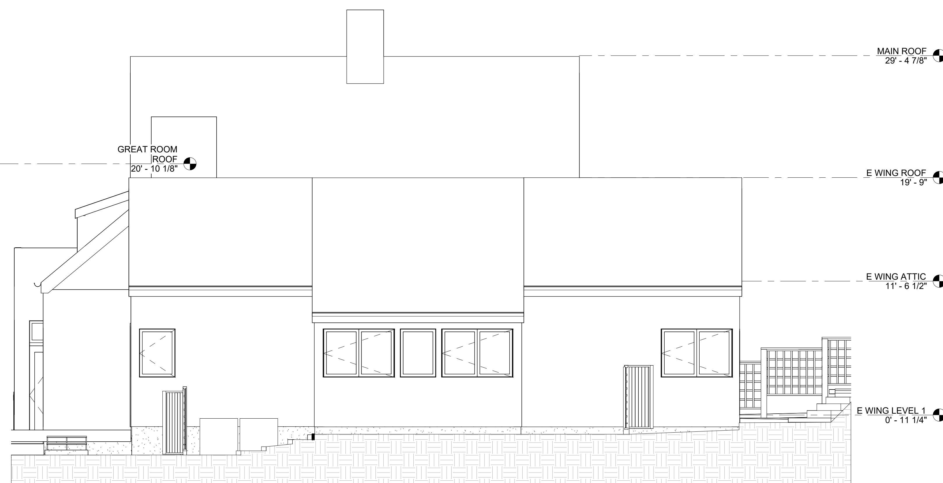
② EAST ELEVATION 1/4" = 1'-0"
