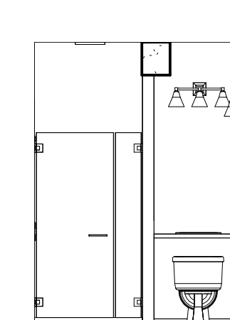
35 GARAGE BATH - SOUTH 1/4" = 1'-0"
