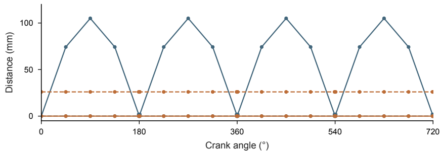
b Maximum centre separation across four cylinders
