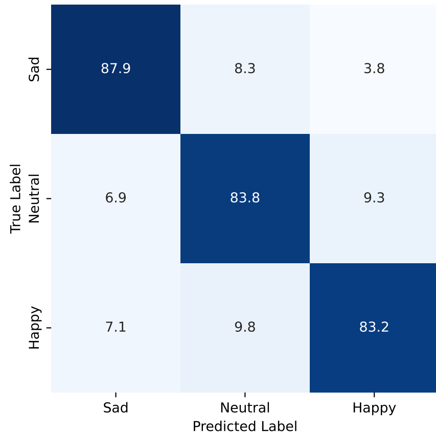
(c) SVM
