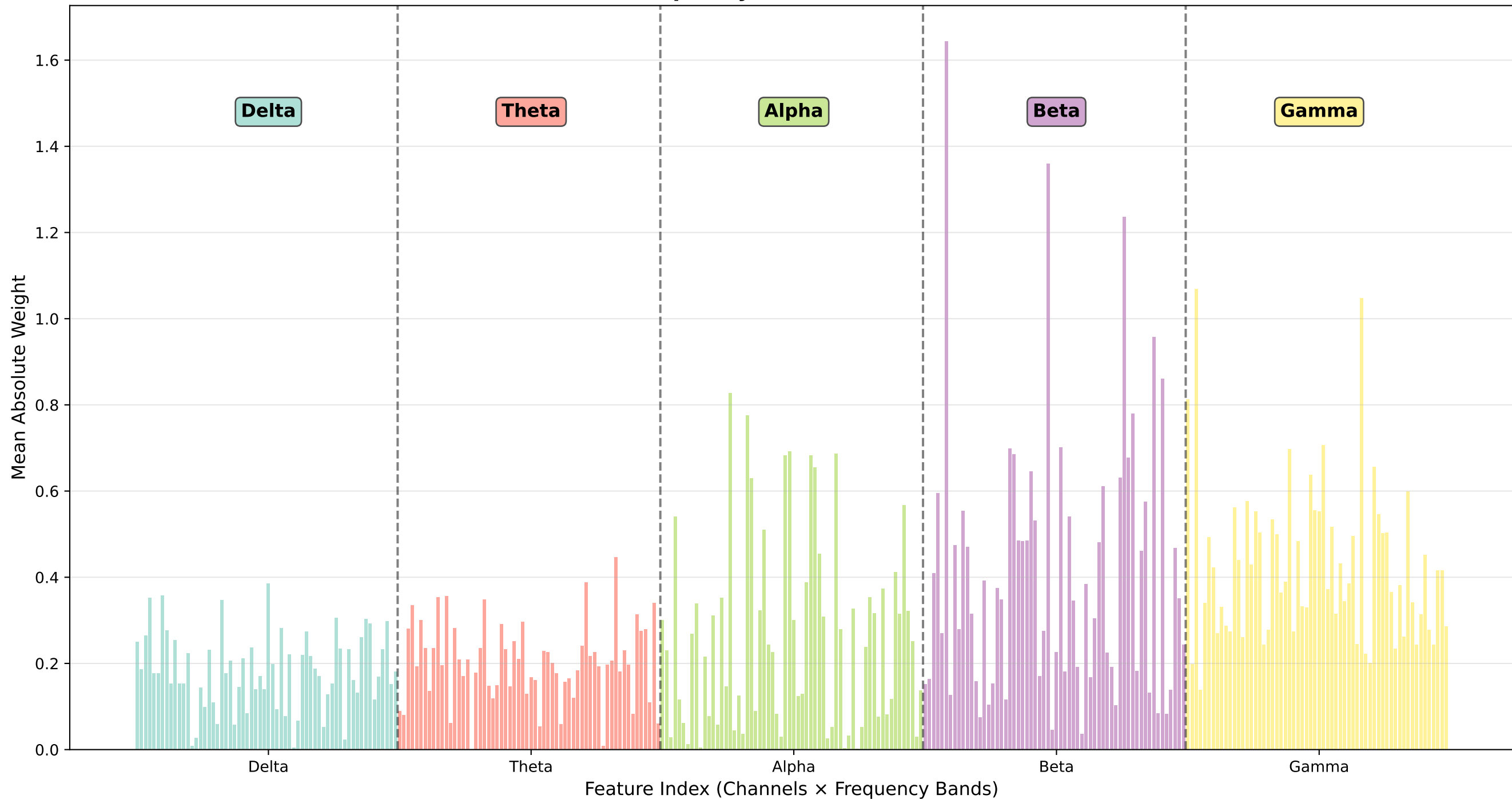
Mean Absolute Weight Distribution of Trained DBNs (Five Frequency Bands Concatenation)
