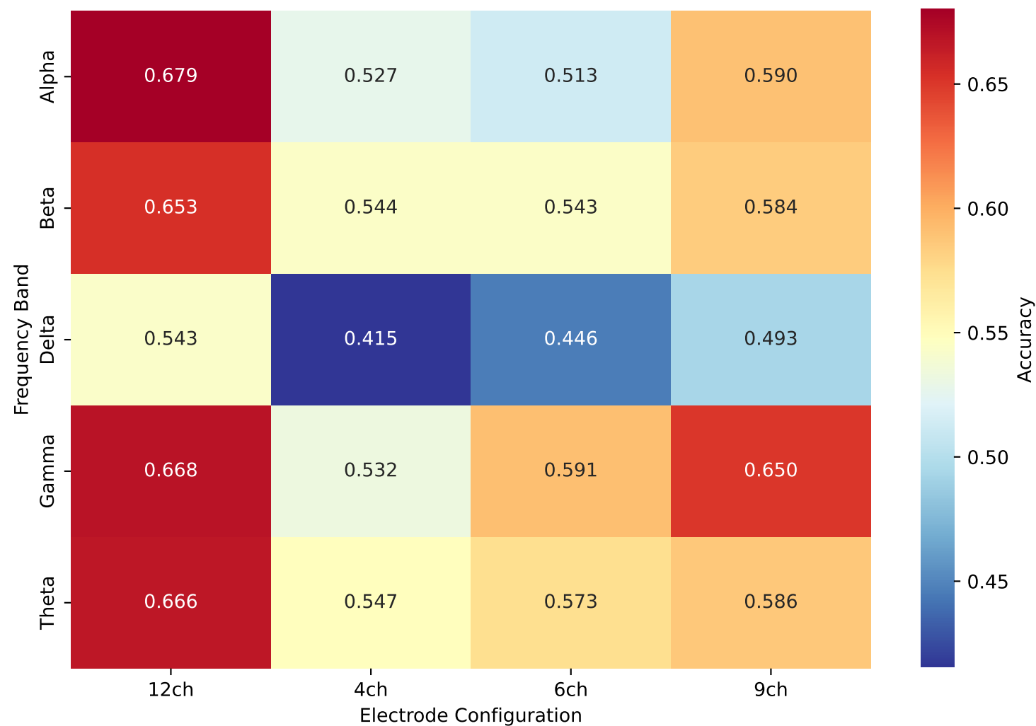
DASM Feature Performance
