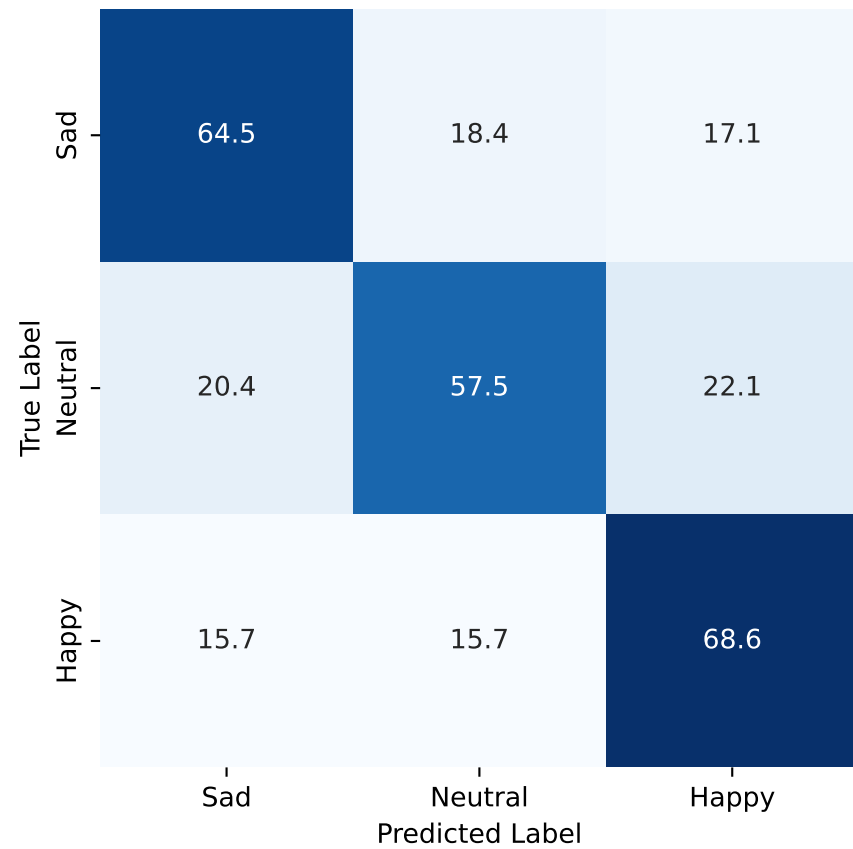
(c) SVM
