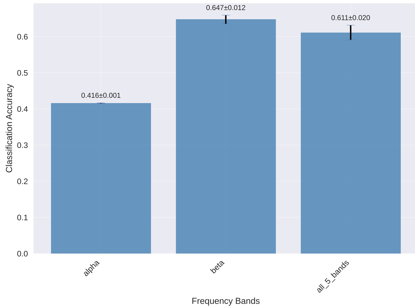
EEG Frequency Band Analysis Classification Performance
