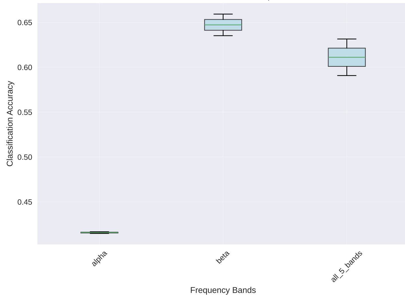
Distribution of Accuracy Scores Across Cross-Validation Repeats
