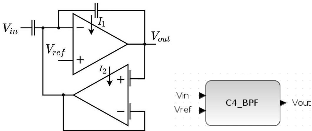
C4 Bandpass Filter:
