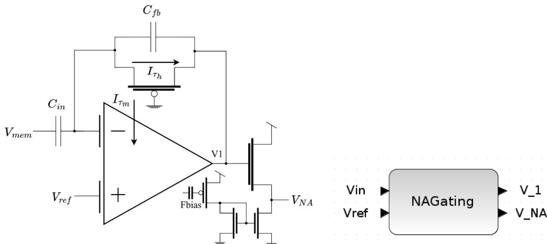
NA Gating Circuit:
