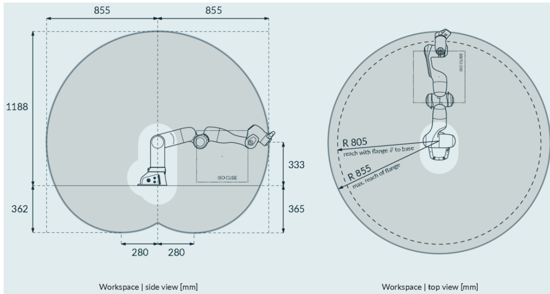
Illustration 4–3 Side and top views of the FR3 workspace envelope. The shared task region is selected inside the overlap of the two practical arm workspaces rather than at the 855 mm reach boundary.
