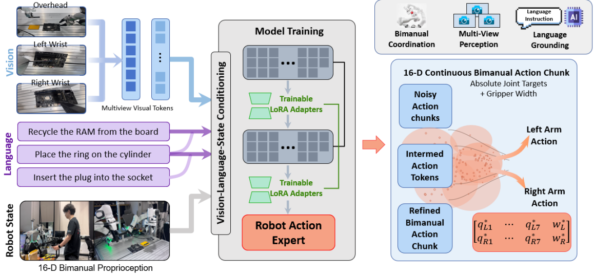
Illustration 4–1 Final \pi_{0.5} model architecture for language-conditioned bimanual manipulation. Multi-view visual observations, a task instruction, and the 16-dimensional bilateral robot state condition the adapted model, which produces continuous action chunks for both FR3 arms and grippers.
