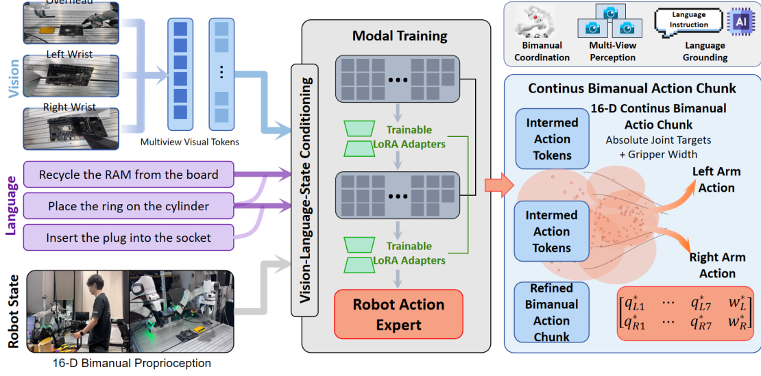
Illustration 4–1 Final \pi_{0.5} model architecture for language-conditioned bimanual manipulation. Multi-view visual observations, a task instruction, and the 16-dimensional bilateral robot state condition the adapted model, which produces continuous action chunks for both FR3 arms and grippers.
