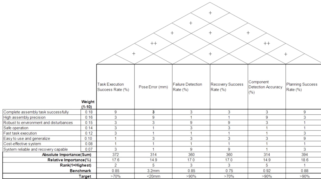
Illustration 2–1 QFD House of Quality for the VLA bimanual manipulation system.
