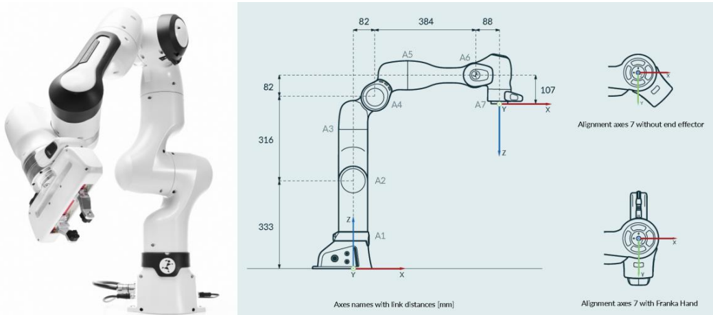
Illustration 4–1 FR3 arm, joint-axis convention, and principal kinematic dimensions retained as a hardware reference.
