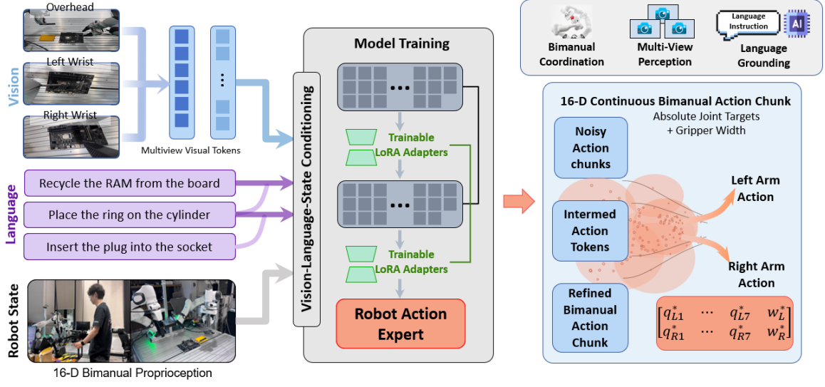
Illustration 4–1 The \pi_{0.5} model architecture for language-conditioned bimanual manipulation. Multi-view visual observations, a task instruction, and the 16-dimensional bilateral robot state condition the adapted model, which produces continuous action chunks for both FR3 arms and grippers.
