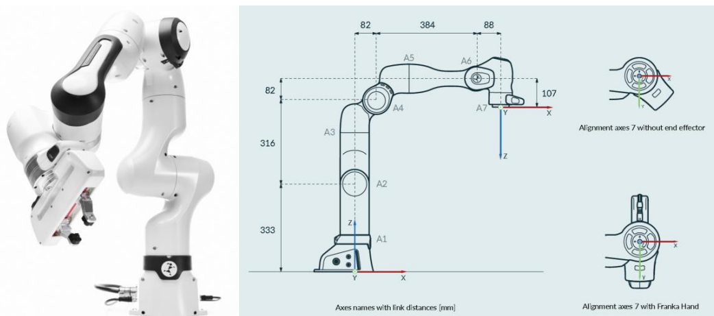
Illustration 7–1 FR3 arm, joint-axis convention, and principal kinematic dimensions retained as a hardware reference.
