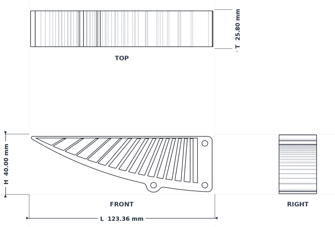
Illustration 61–4 Orthographic views of one TPU 64D compliant gripper finger and its overall dimensions.
