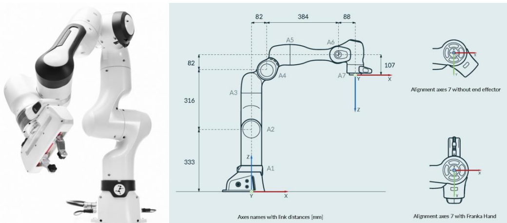
Illustration 12–1 FR3 arm, joint-axis convention, and principal kinematic dimensions retained as a hardware reference.
