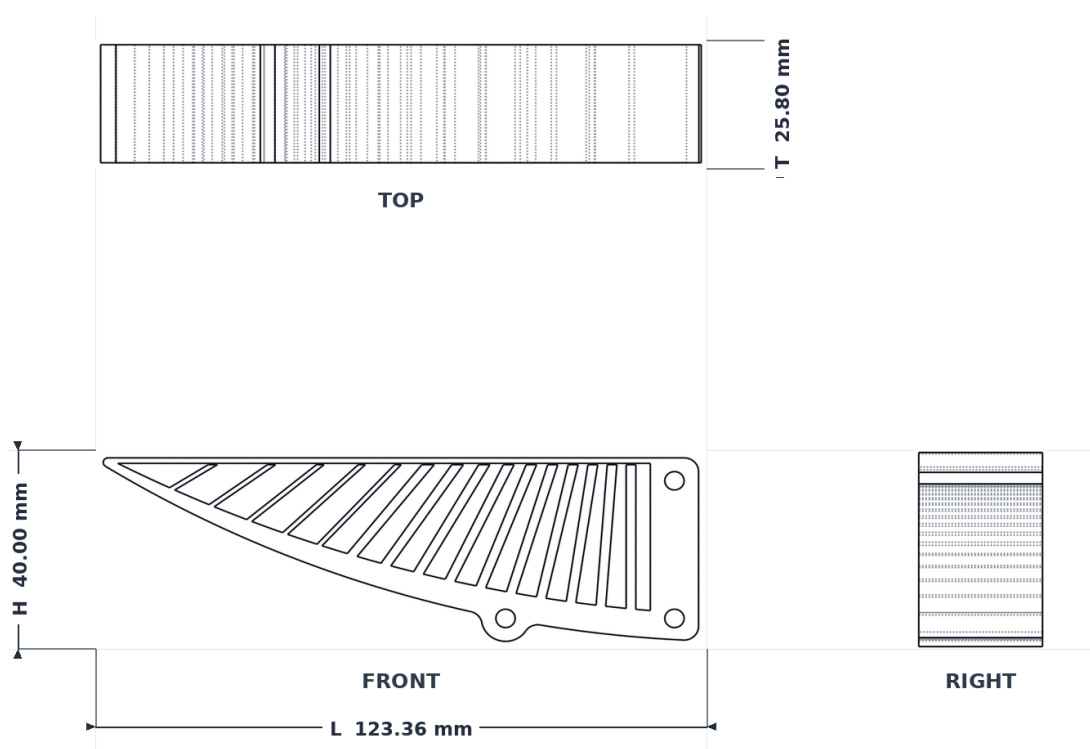
Illustration 9–4 Orthographic views of one TPU 64D compliant gripper finger and its overall dimensions.
