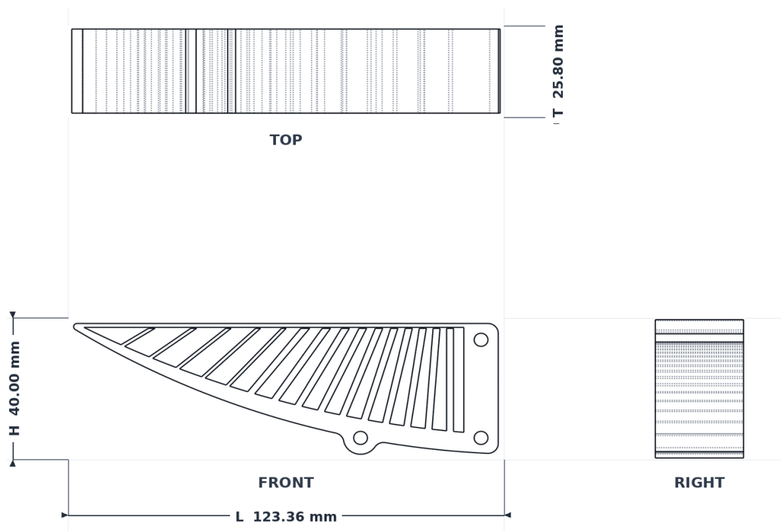
Illustration 58–4 Orthographic views of one TPU 64D compliant gripper finger and its overall dimensions.
