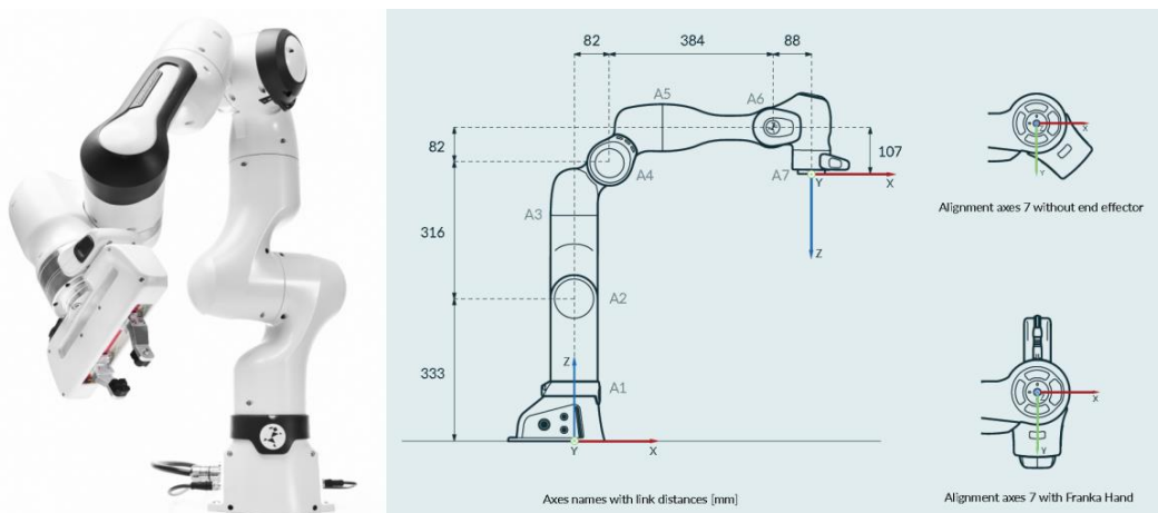
Illustration 42–1 FR3 arm, joint-axis convention, and principal kinematic dimensions retained as a hardware reference.
