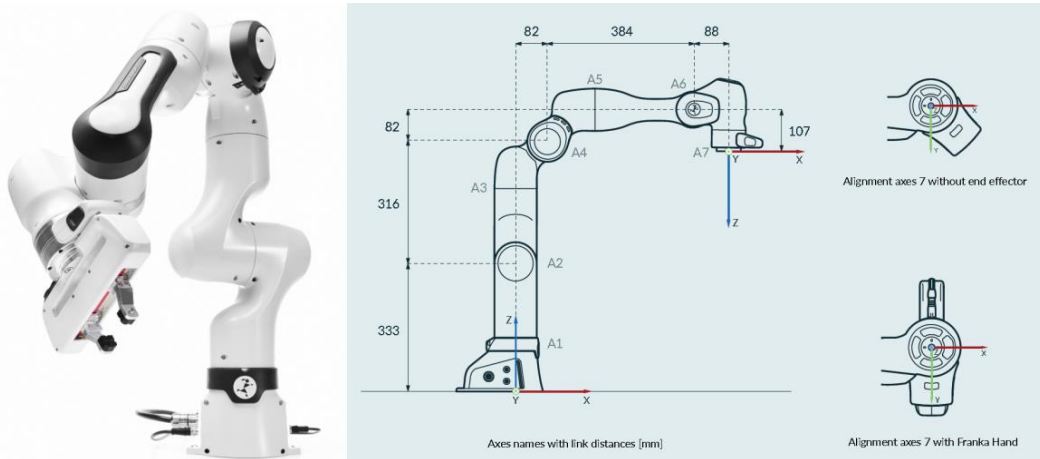
Illustration 45–1 FR3 arm, joint-axis convention, and principal kinematic dimensions retained as a hardware reference.
