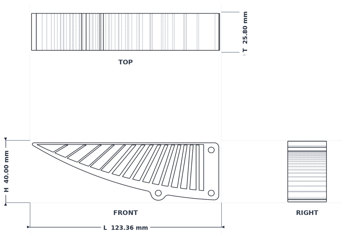
Illustration 56-4 Orthographic views of one TPU 64D compliant gripper finger and its overall dimensions.
