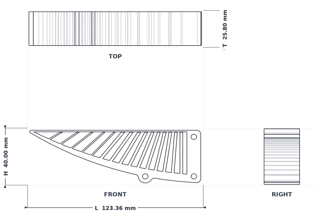
Illustration 20–4 Orthographic views of one TPU 64D compliant gripper finger and its overall dimensions.
