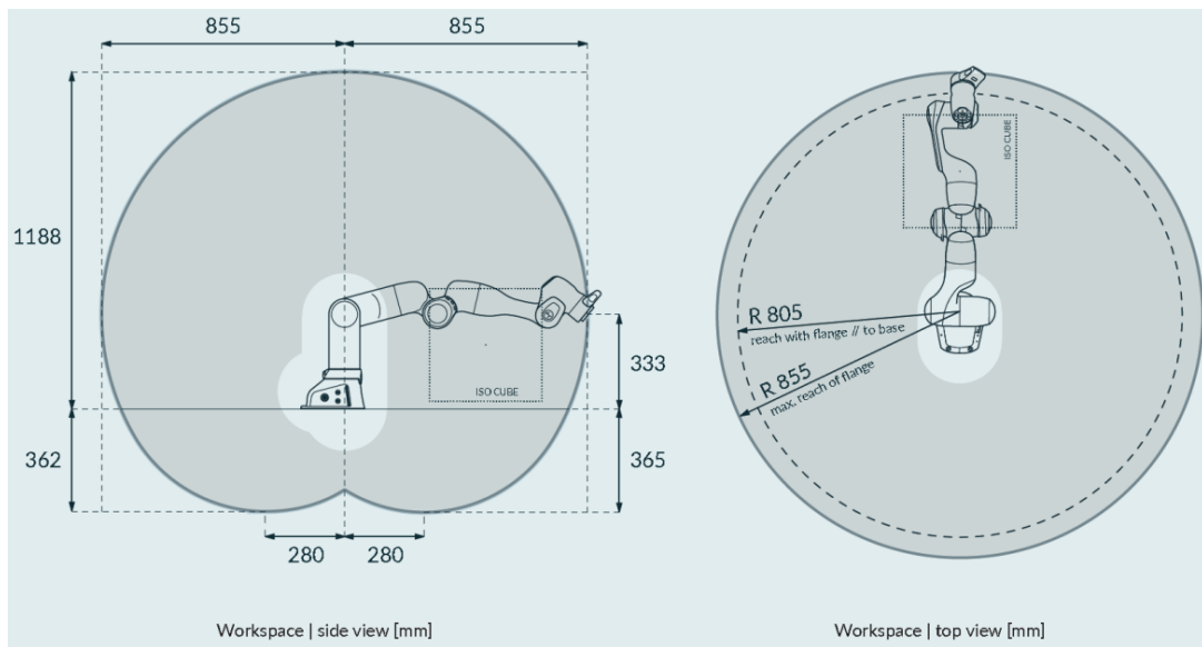
Illustration 5–2 Side and top views of the FR3 workspace envelope. The shared task region is selected inside the overlap of the two practical arm workspaces rather than at the 855 mm reach boundary.
