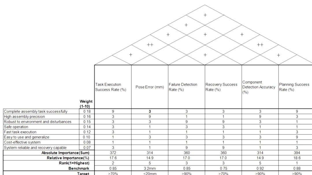
Illustration 2-1 QFD House of Quality for the VLA bimanual manipulation system.
