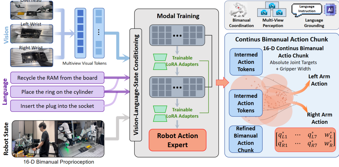
Illustration 4-1 Final language-conditioned \pi_{0.5} architecture. Three RGB views, a task instruction, and 16-dimensional bimanual proprioception condition the unified model. Trainable LoRA adapters and the robot action expert generate continuous 16-dimensional action chunks containing absolute joint targets and gripper widths for the left and right arms.
