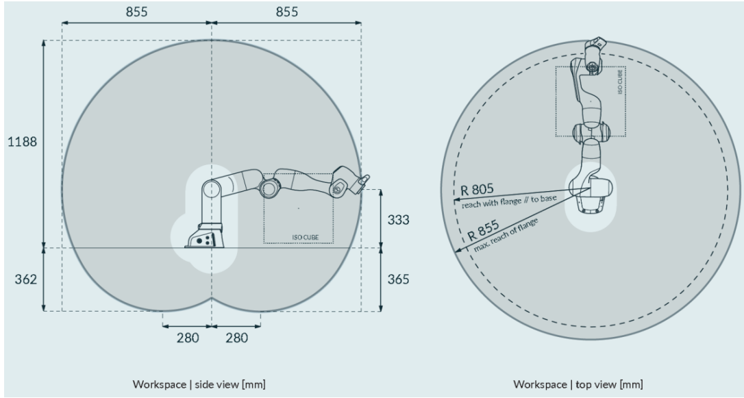
Illustration 4–2 Side and top views of the FR3 workspace envelope. The shared task region is selected inside the overlap of the two practical arm workspaces rather than at the 855 mm reach boundary.
