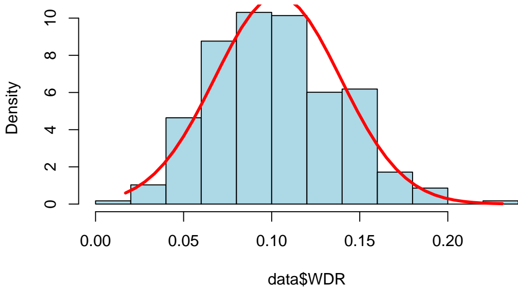
Histogram of data$WDR
