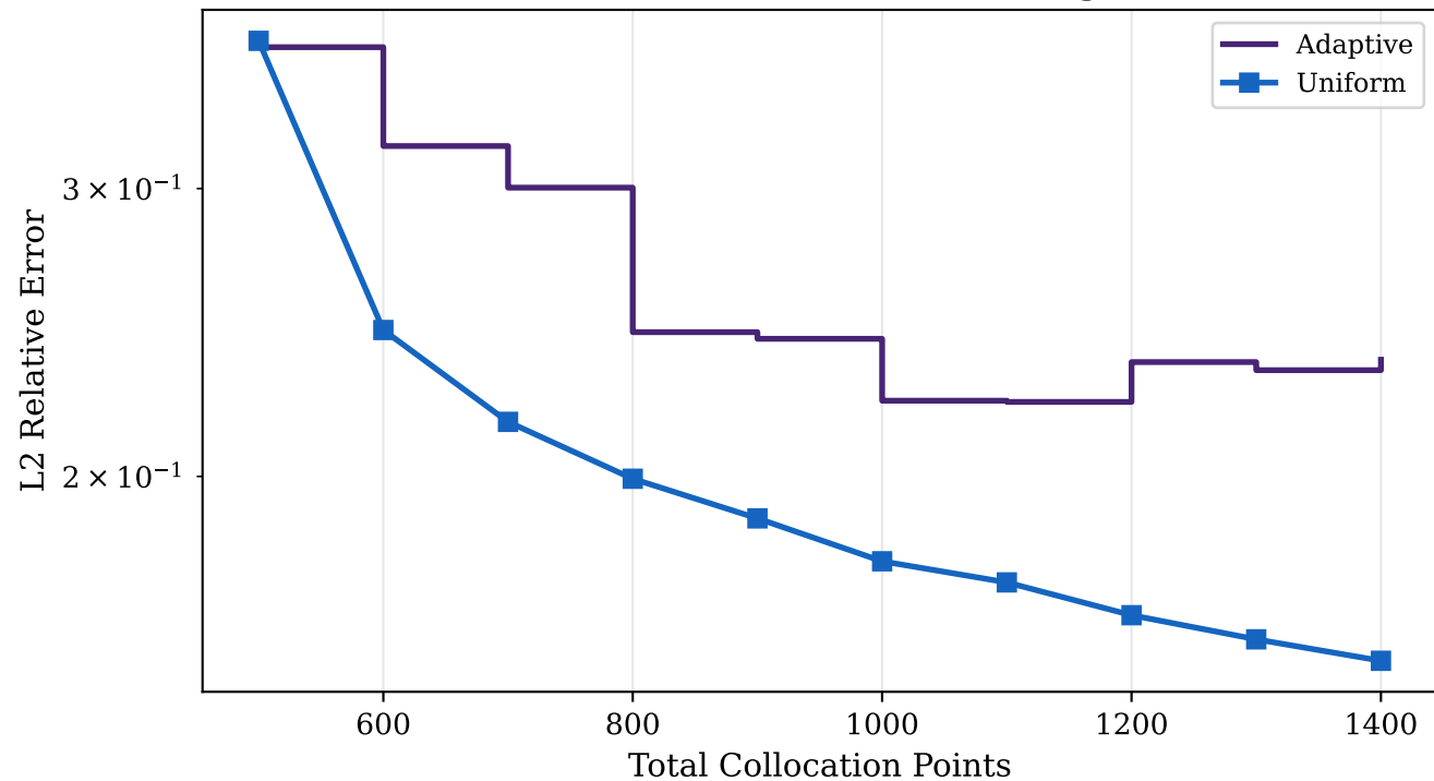
L2 Error vs Total Point Budget
