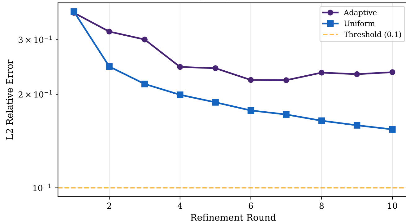
Adaptive vs Uniform Growth (Both start at 500 pts, pre-trained 5000 epochs)
