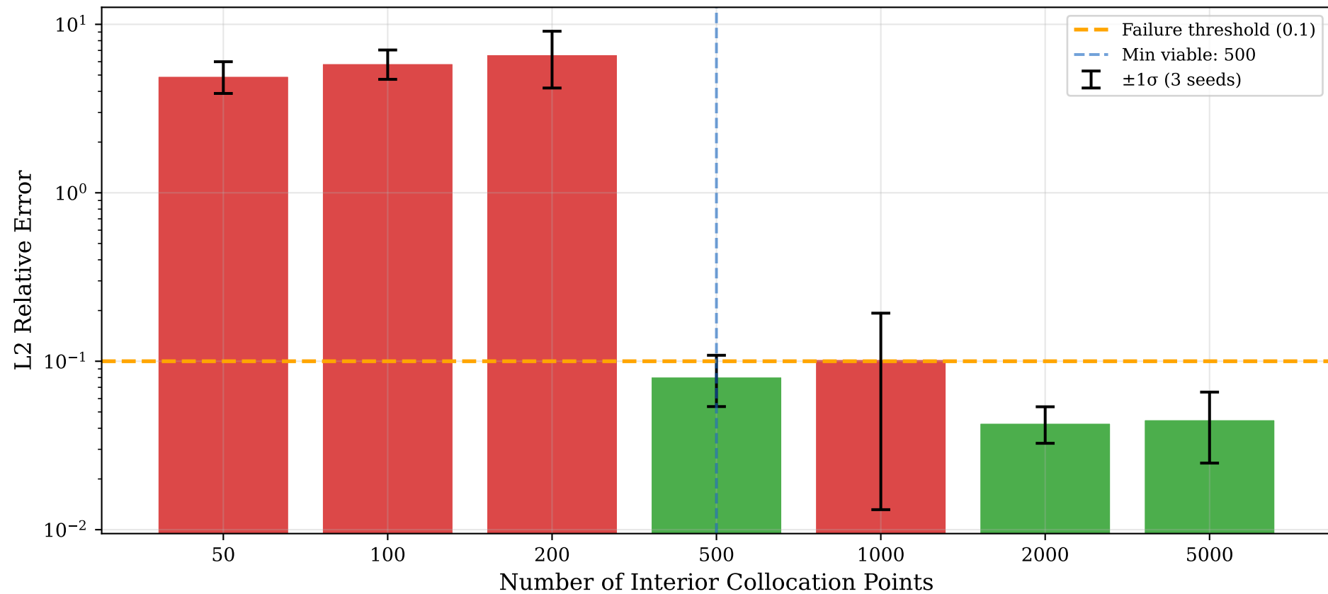
L2 Error vs Collocation Count (mean \pm \sigma , 3 seeds)
