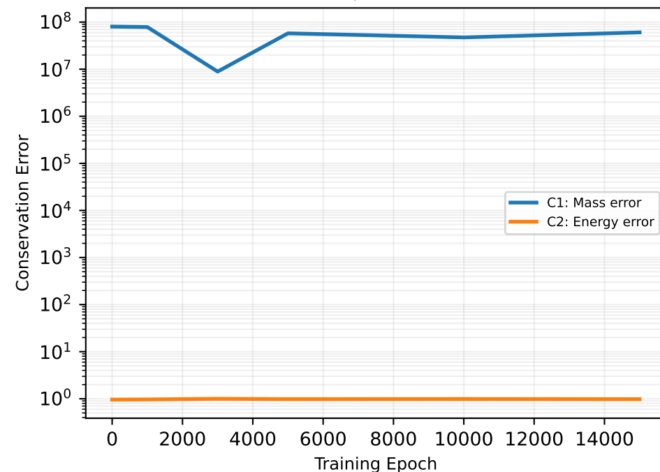
FM4: Viscous Shock ( \nu=0.1 )
