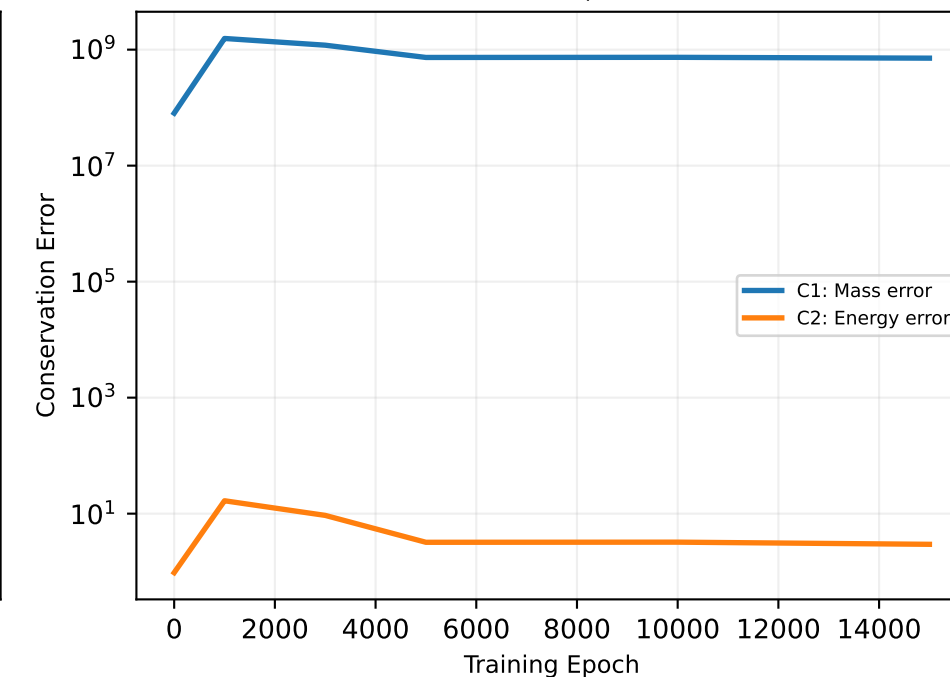
FM5: Collocation Starvation ( \beta=10 )
