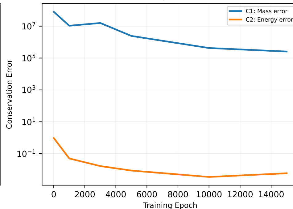
FM5: Collocation Starvation ( \beta=10 )
