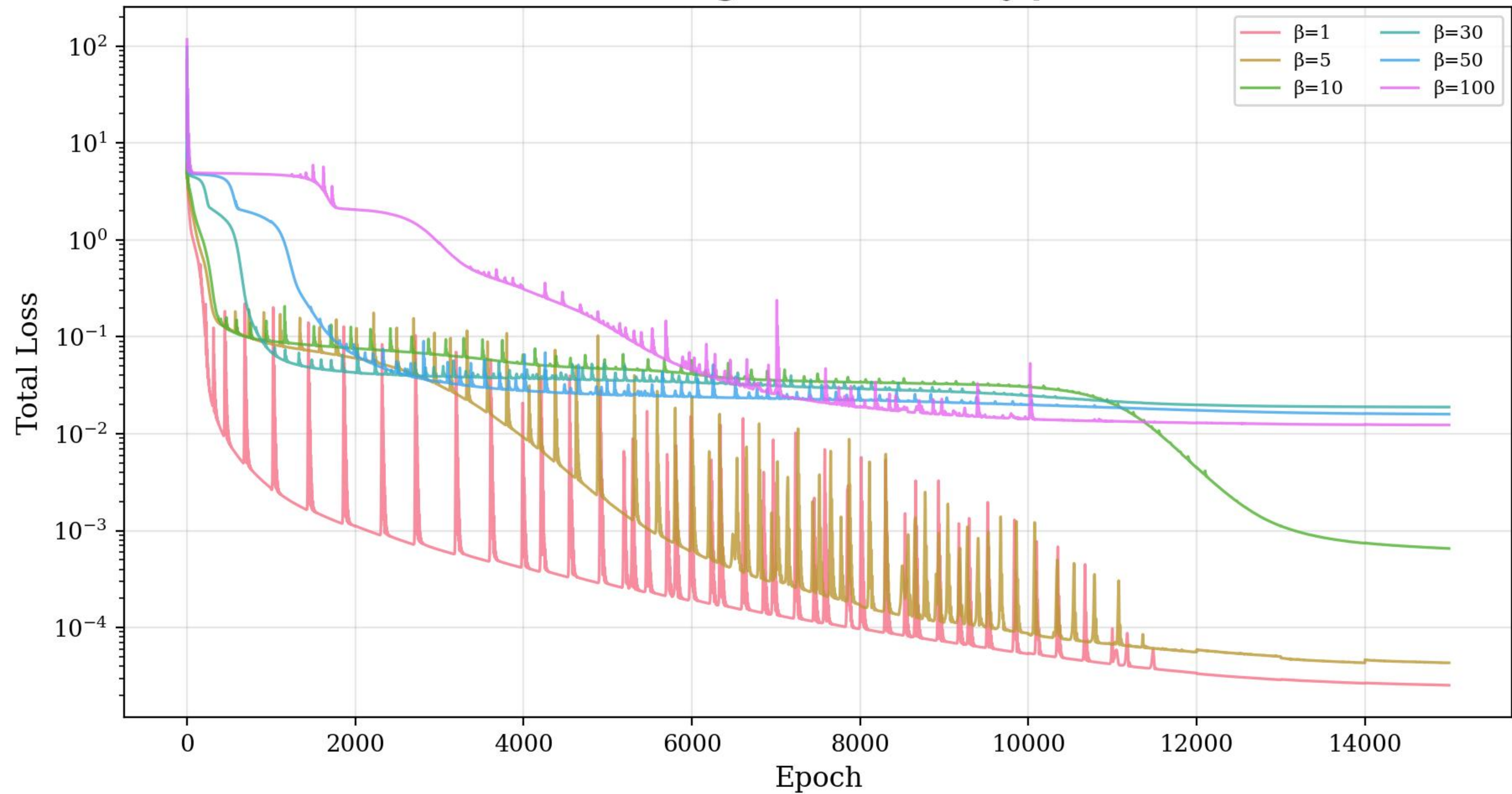
Training Loss Curves by \beta
