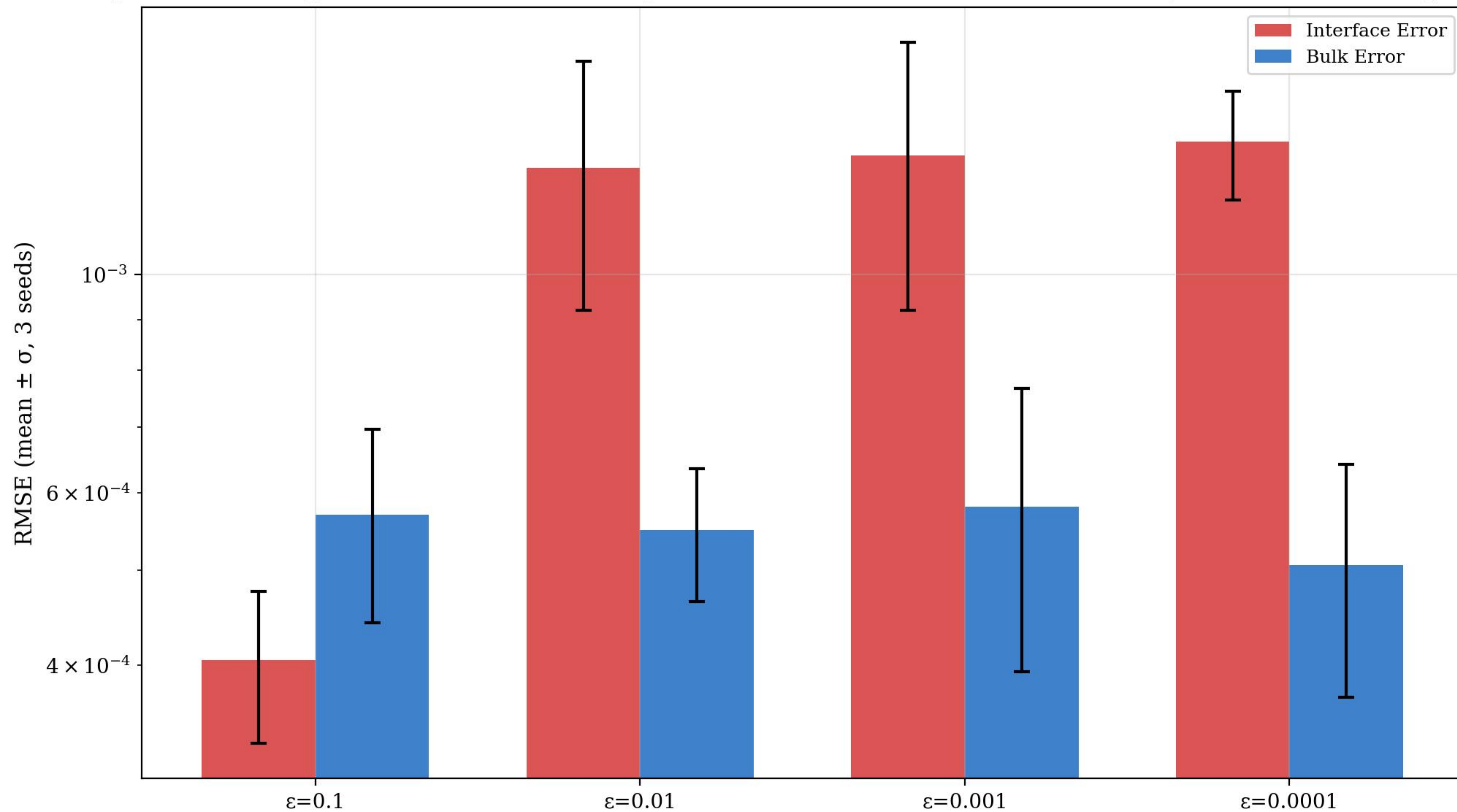
Interface vs Bulk Error by \varepsilon Spectral bias signature: interface error grows faster than bulk as \varepsilon decreases (even in success regime).
