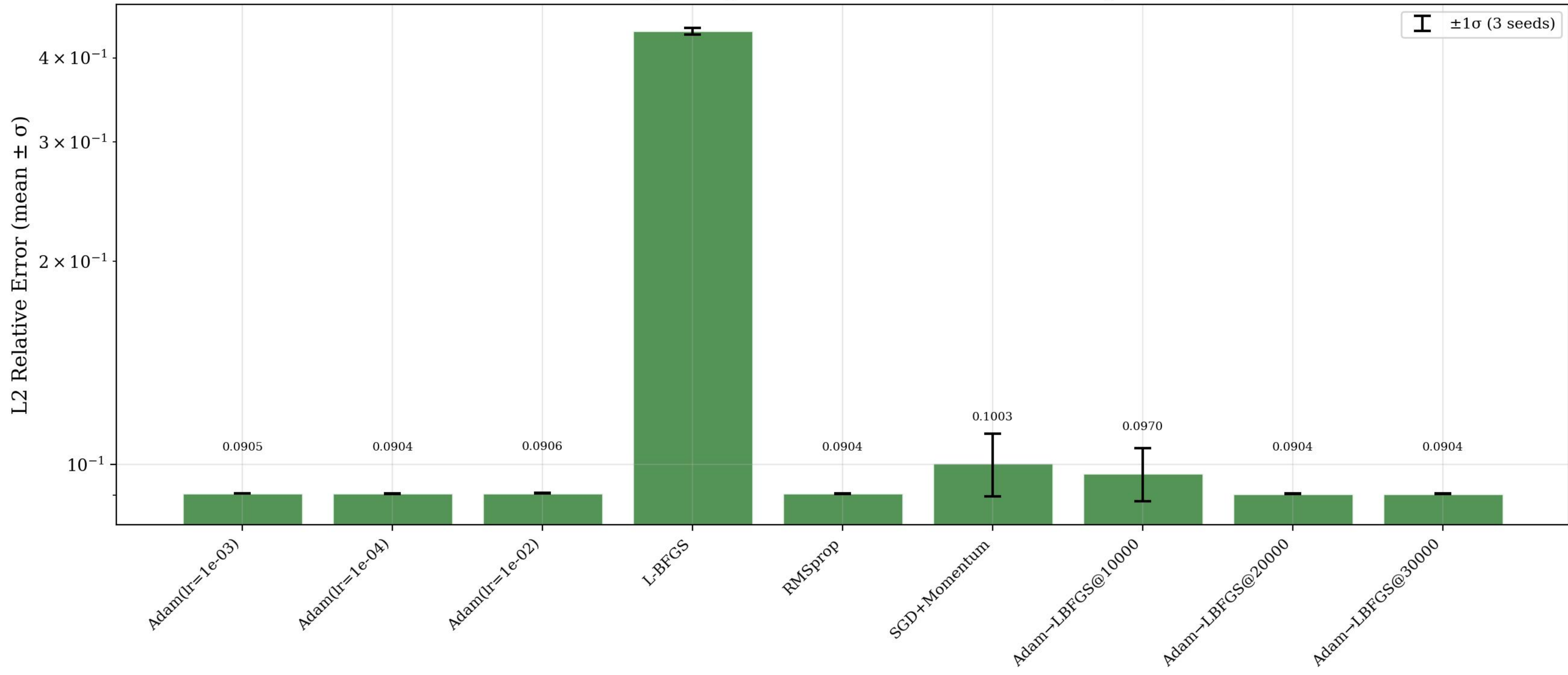
Final L2 Error by Optimizer Green=success Orange=stagnation Red=ill-conditioned Purple=divergence
