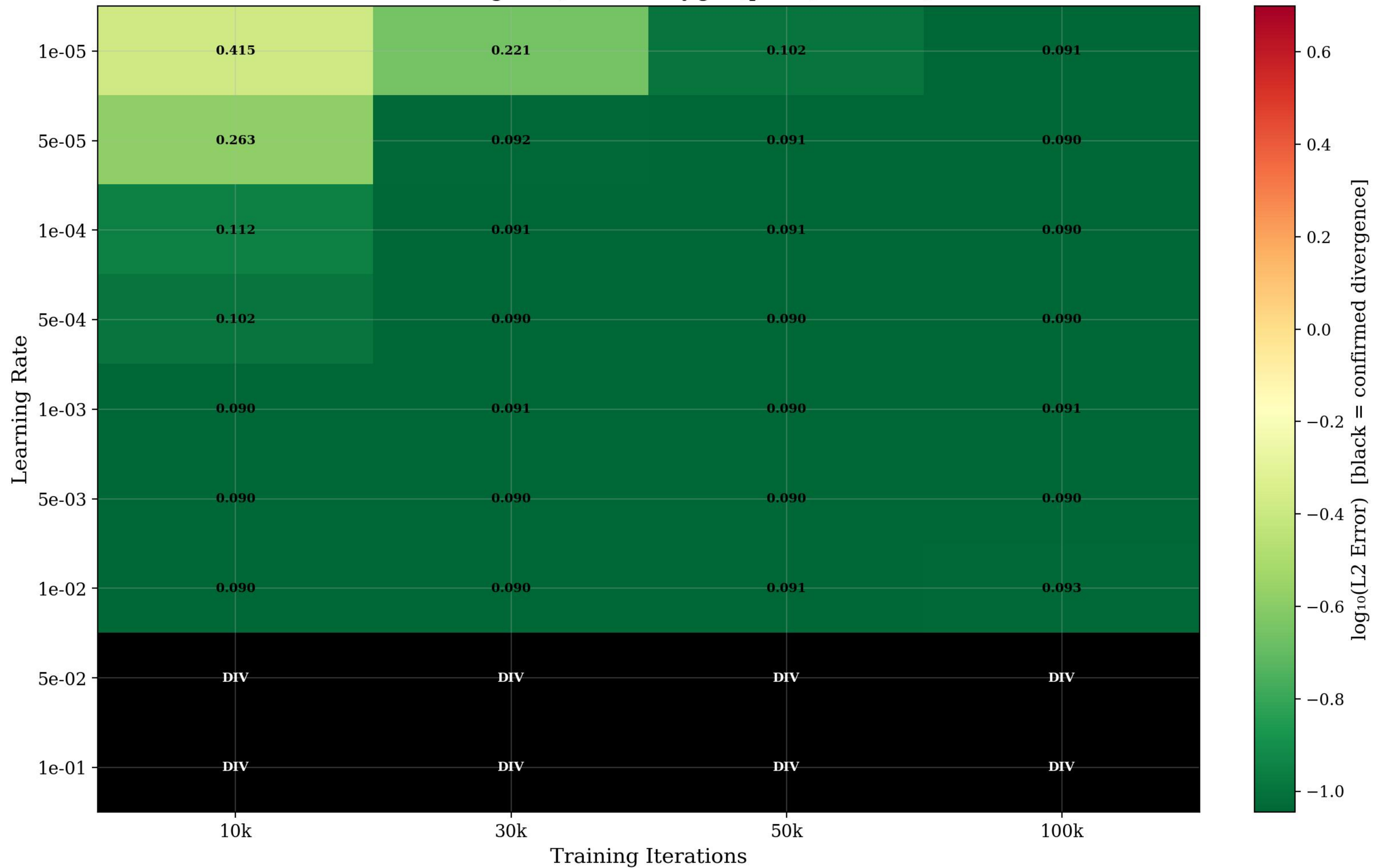
Learning Rate × Iterations Phase Diagram Black = divergence (confirmed by grad/param/loss norms).
