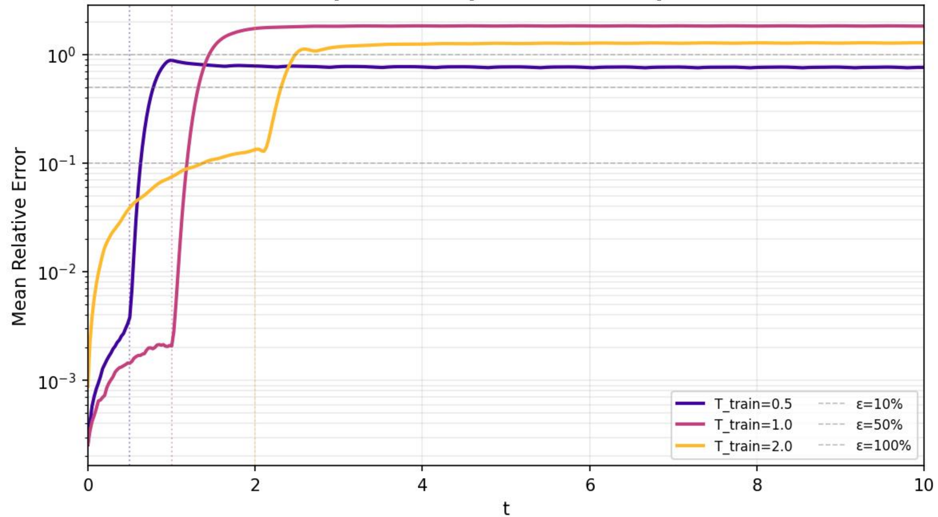
Temporal Extrapolation Error ( \beta=10 )
