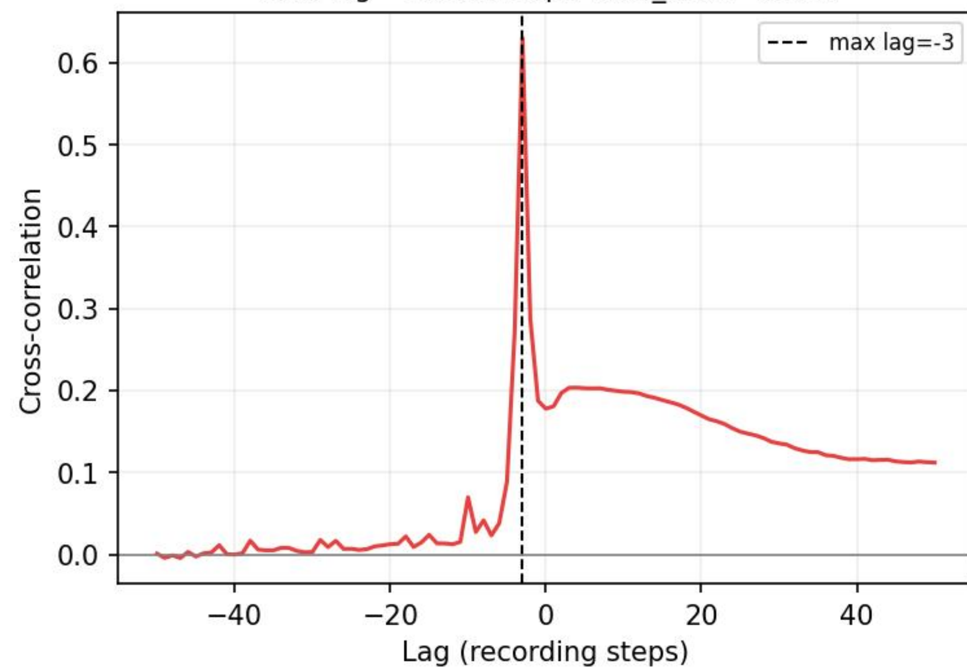
Spectral \leftrightarrow Gradient Cross-correlation Peak lag=-3 \times 200 steps max_xcorr=0.630
