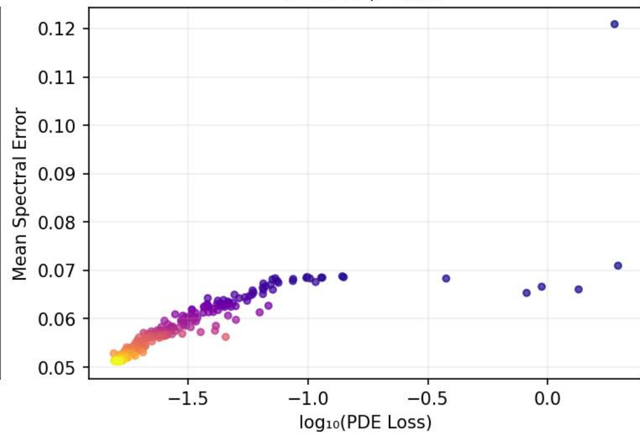
PDE Loss vs Spectral Error r=0.842 p=0.000
