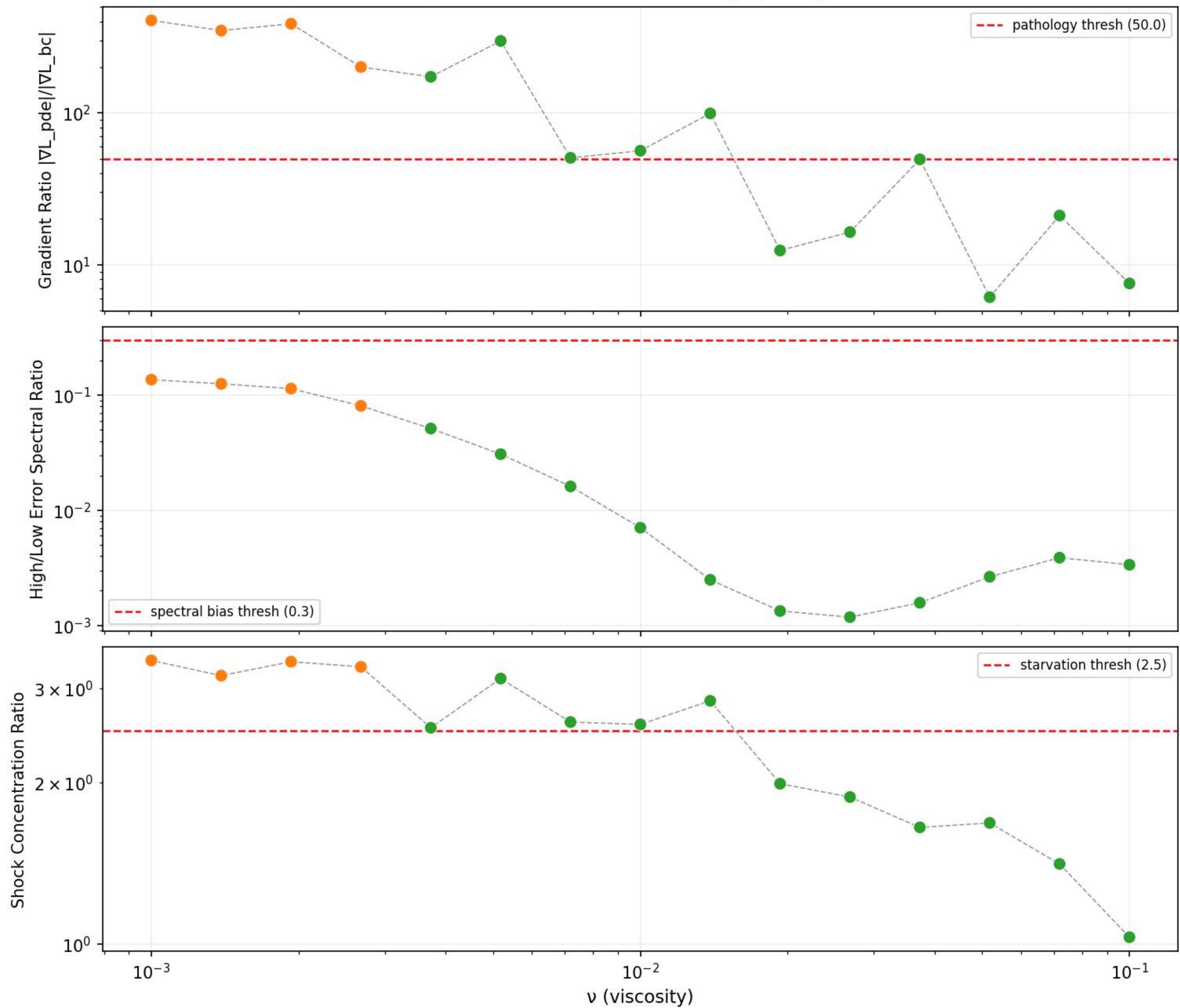
Diagnostic Signals vs Viscosity \nu (FIX 4: spectral ratio uses error FFT / \|u_{\text{exact}}\|_2 )
