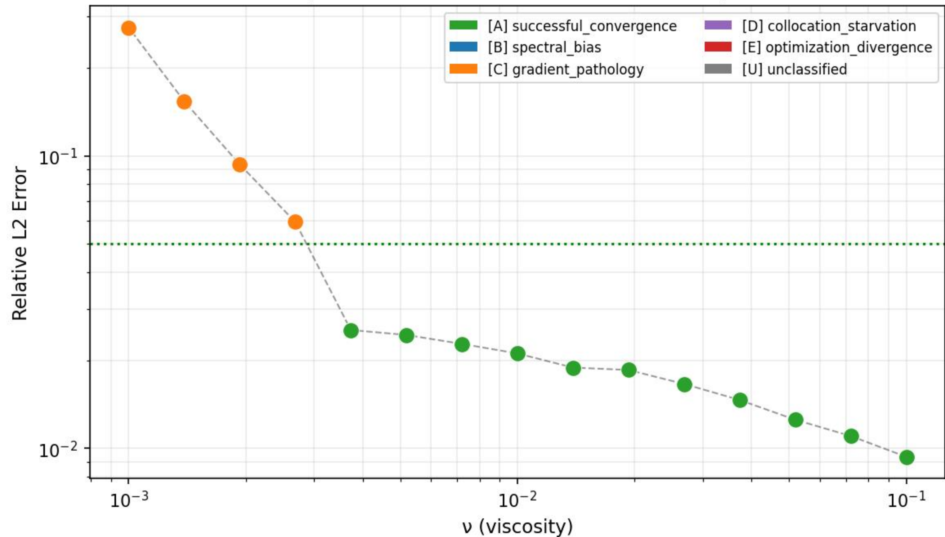
L2 Error vs Viscosity \nu — Burgers PINN (colors = failure mode classification)
