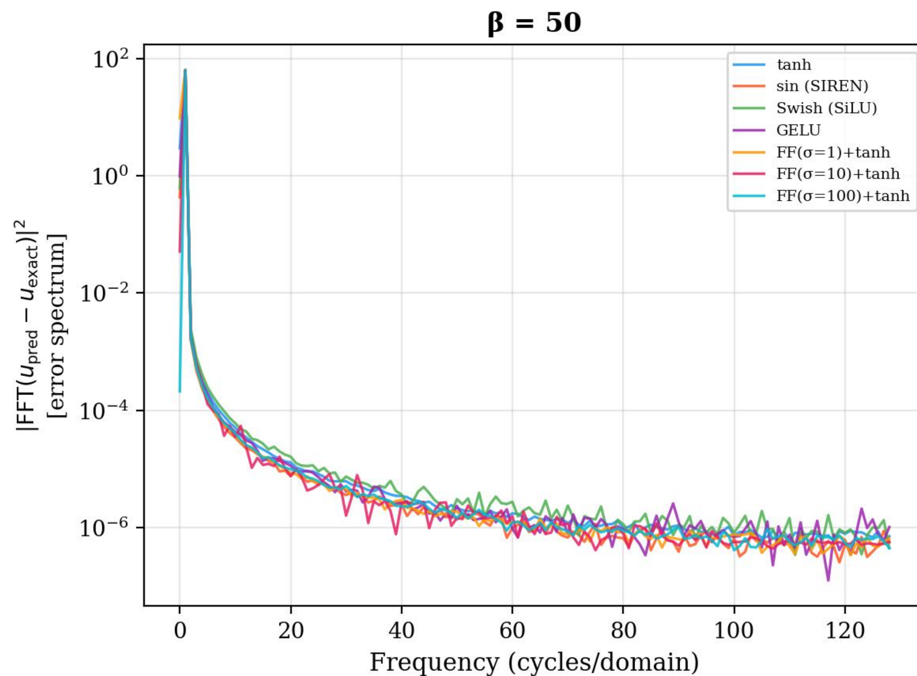
Spectral Error Distribution by Activation Function (y-axis: pointwise error spectrum, not solution spectrum — cf. Exp 1 spectral_comparison.png)
