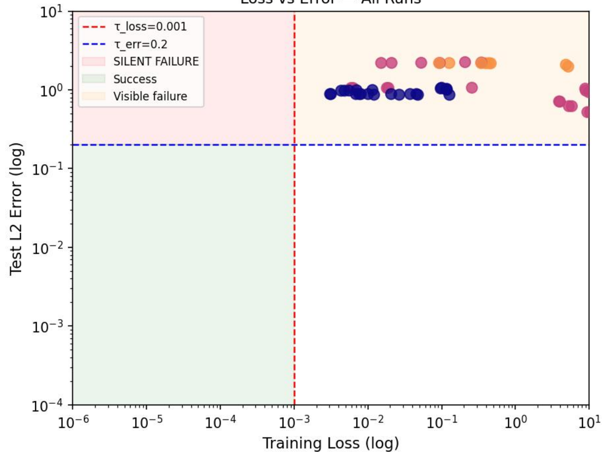
Loss vs Error — All Runs
