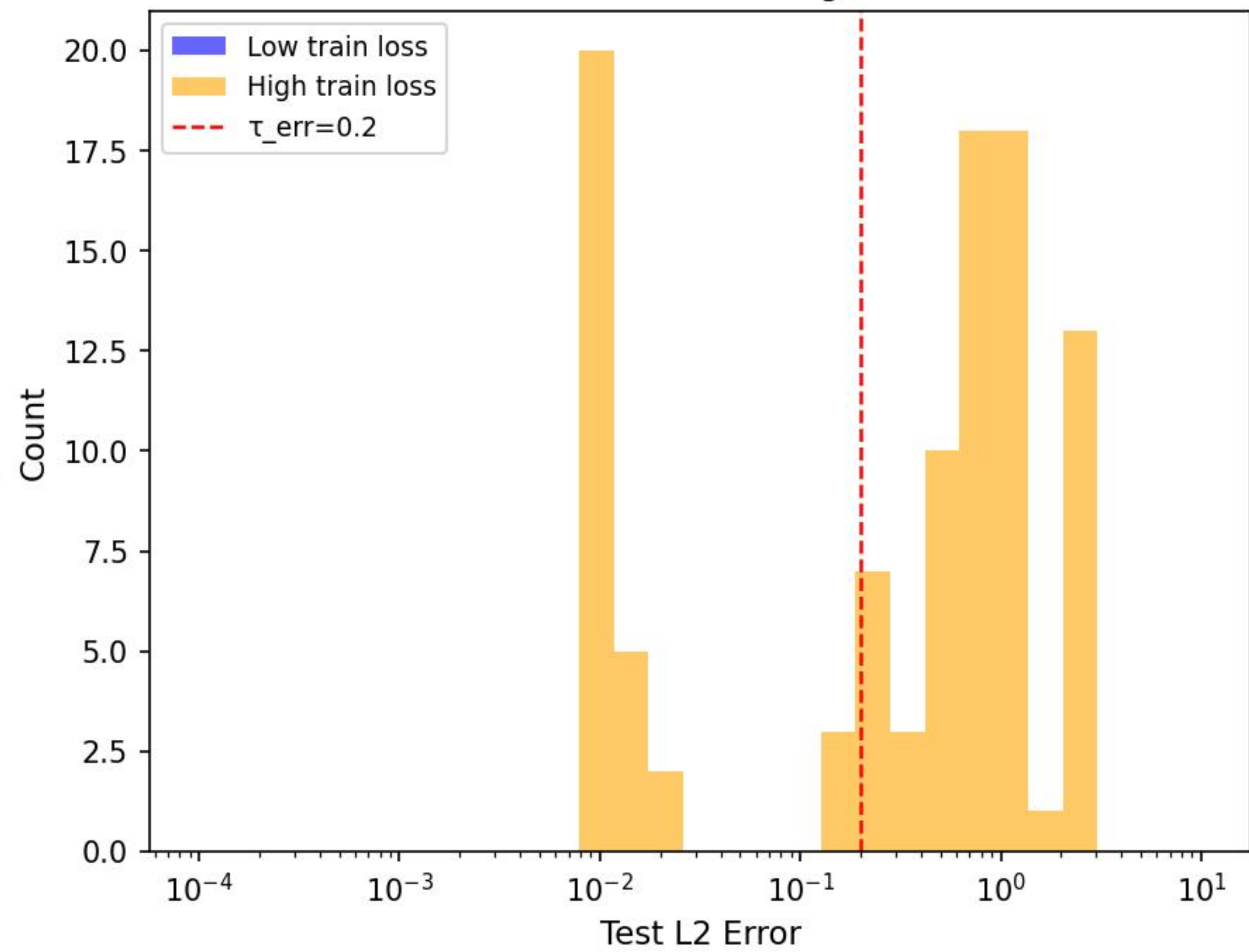
Error Distribution: Converged vs Not
