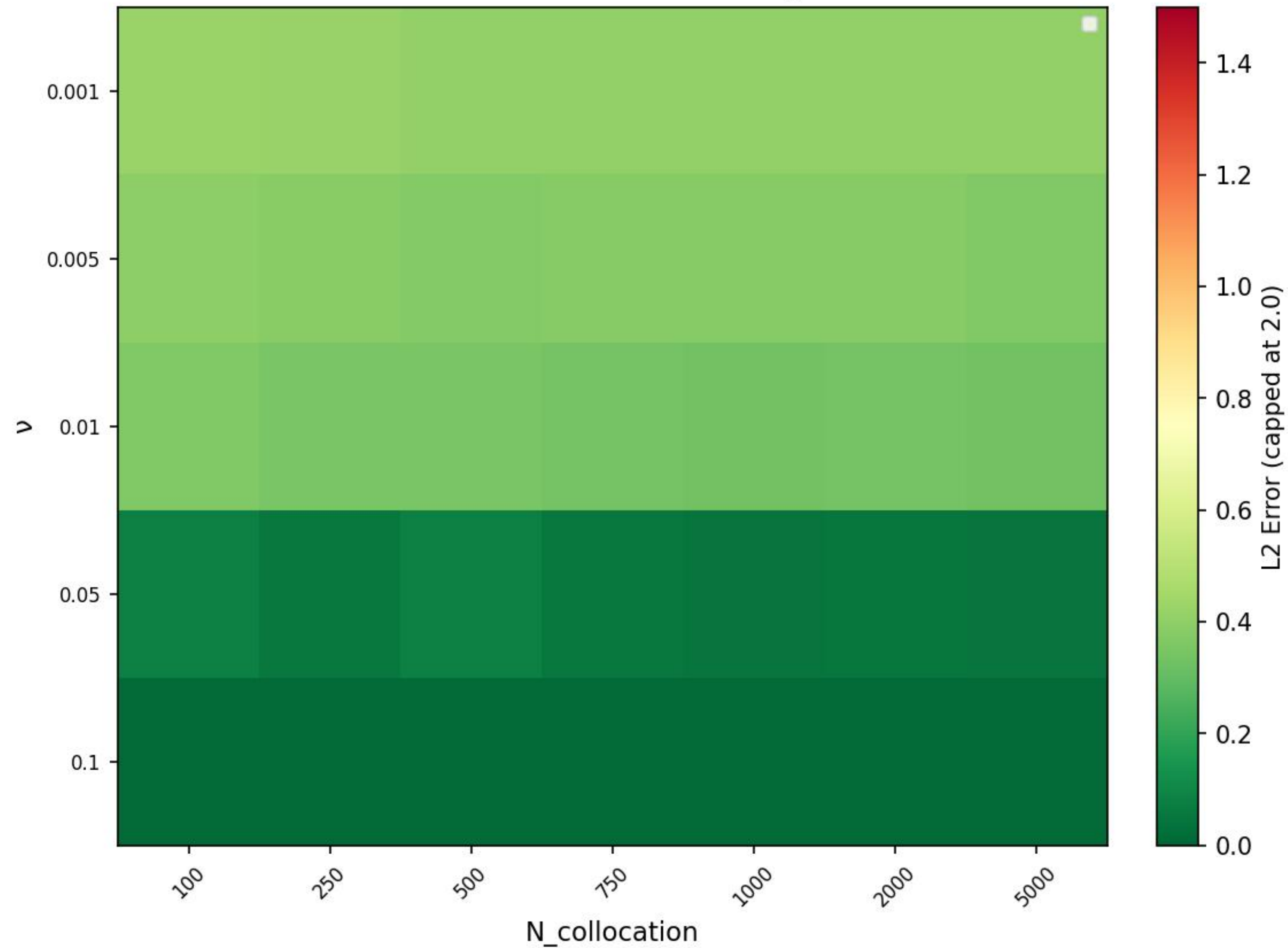
L2 Error + Success Boundary
