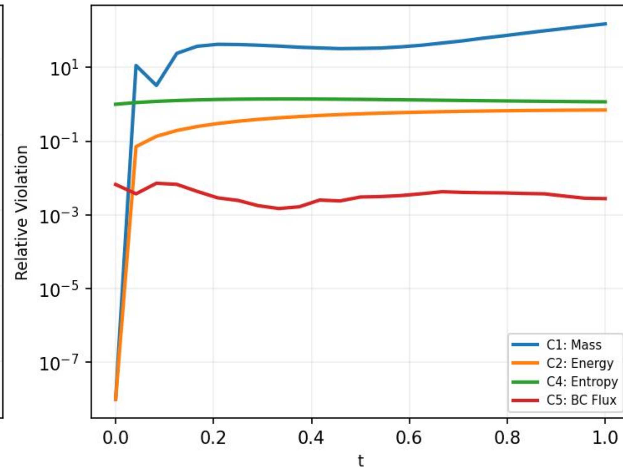
FM5: Collocation Starvation (N=200) L2=0.4156
